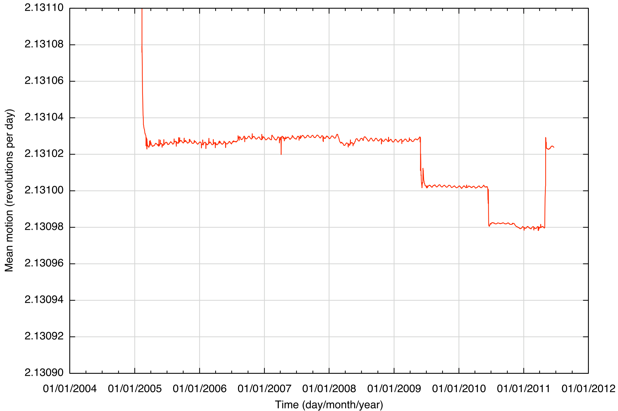
GLONASS 712 Mean Motion from NORAD Two-Line Mean Elements
