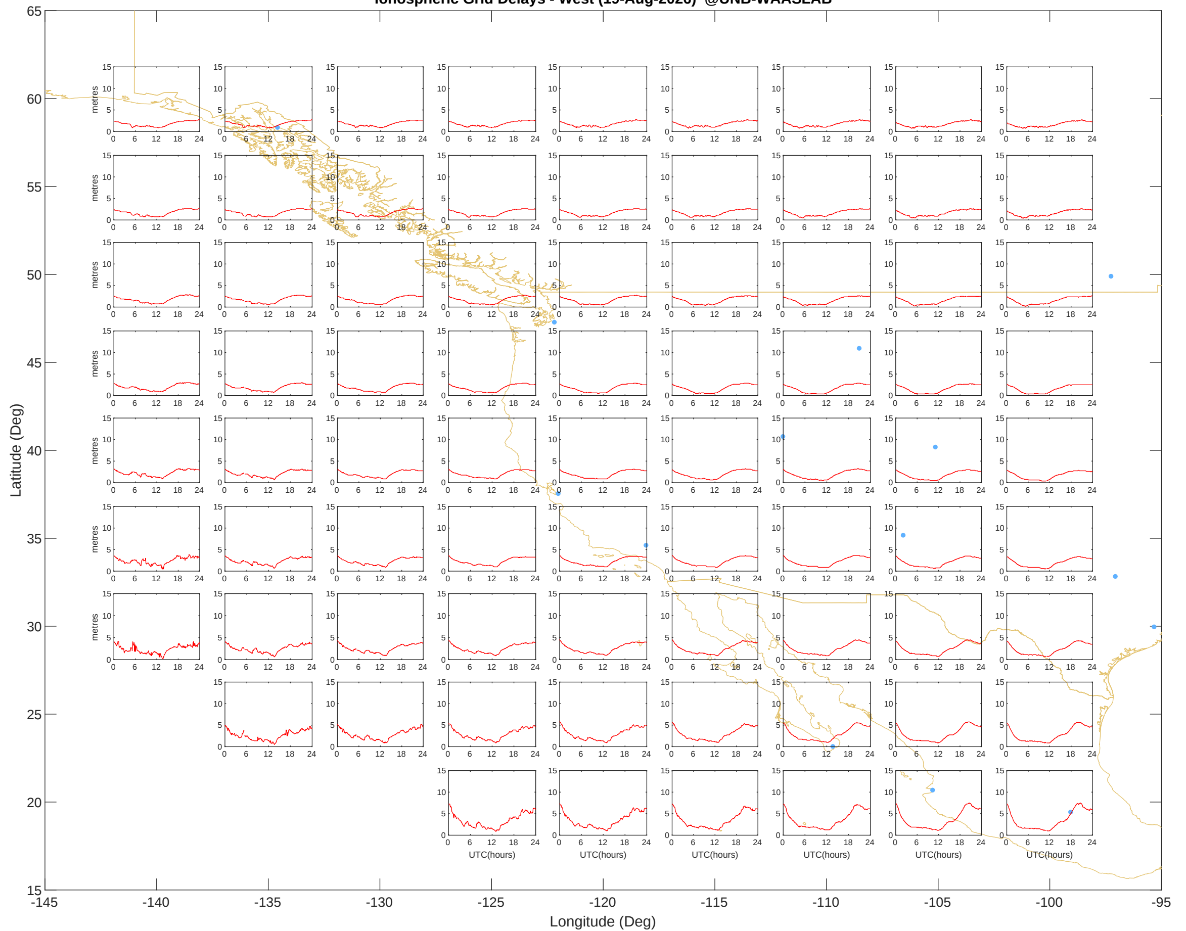
Ionospheric Grid Delays - West (19-Aug-2026) @UNB-WAASLAB
