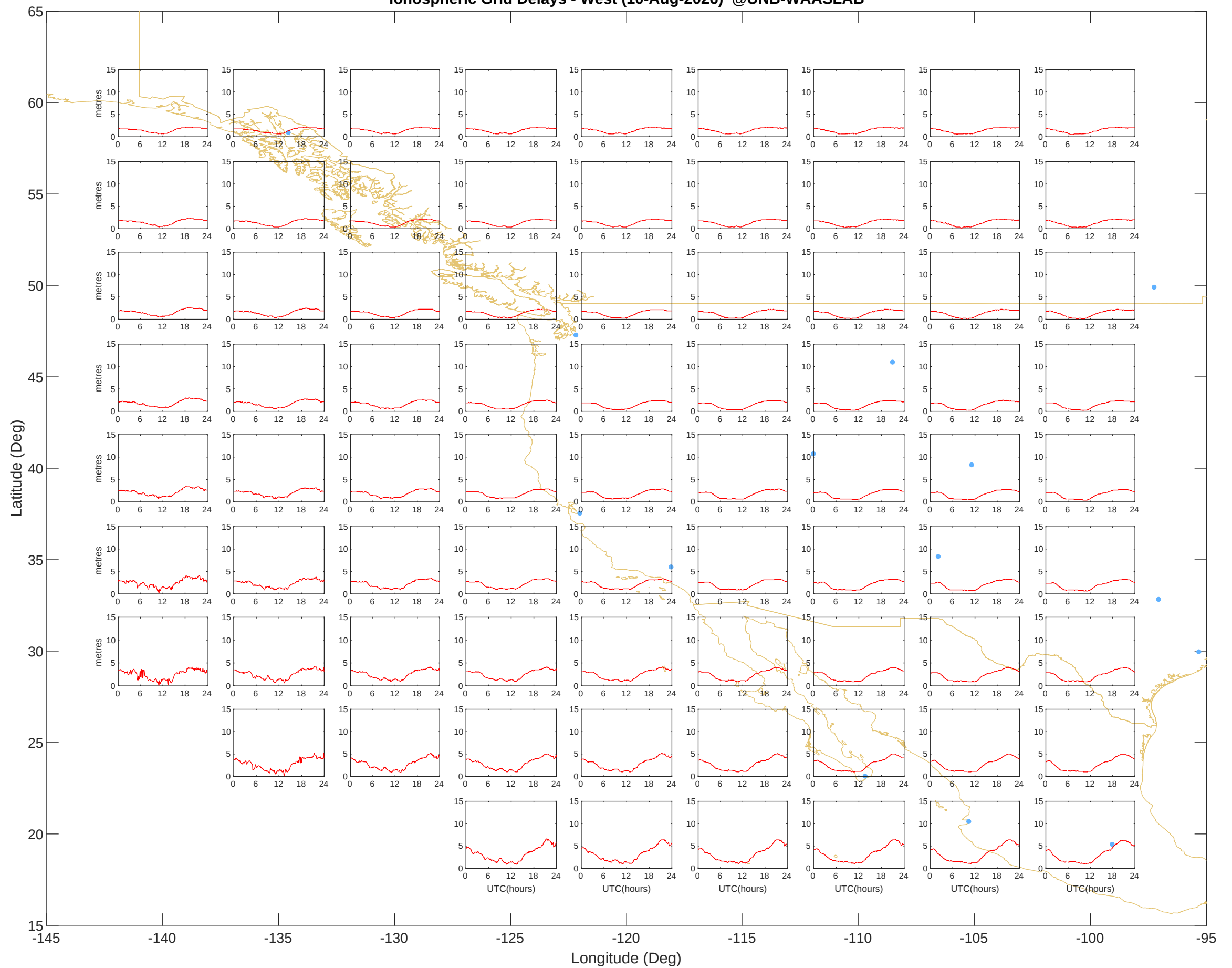
Ionospheric Grid Delays - West (10-Aug-2026) @UNB-WAASLAB
