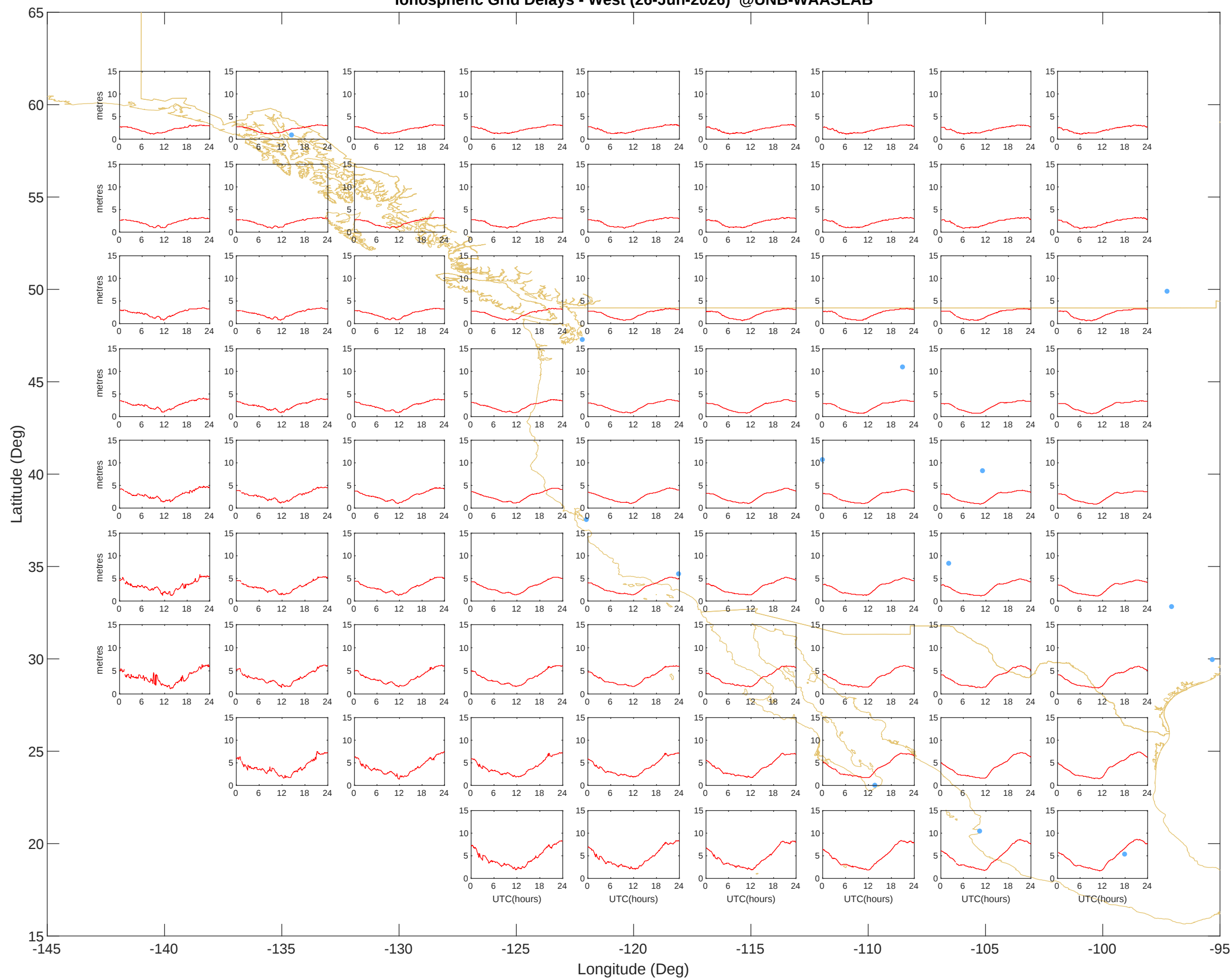
Ionospheric Grid Delays - West (26-Jun-2026) @UNB-WAASLAB
