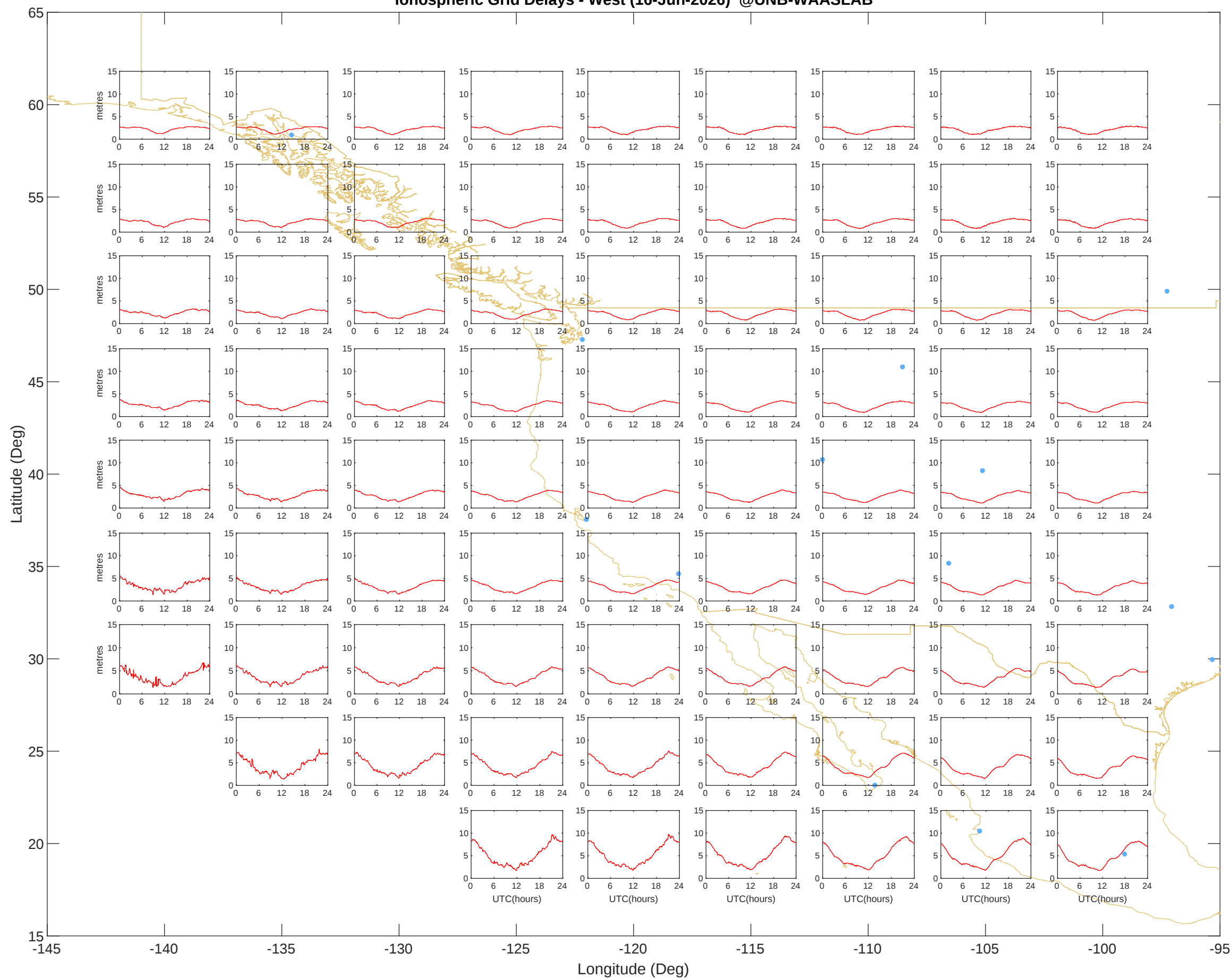
Ionospheric Grid Delays - West (16-Jun-2026) @UNB-WAASLAB
