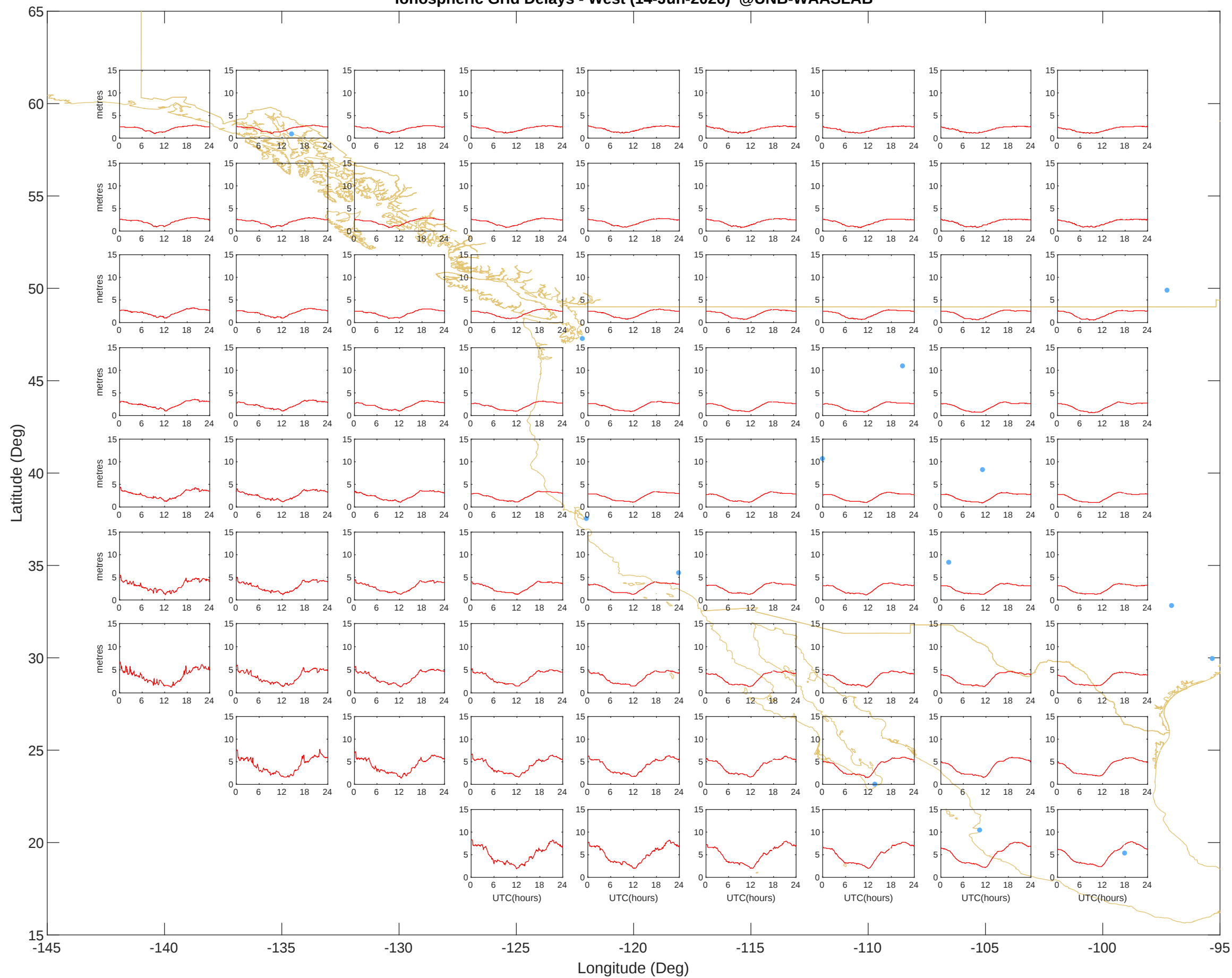
Ionospheric Grid Delays - West (14-Jun-2026) @UNB-WAASLAB
