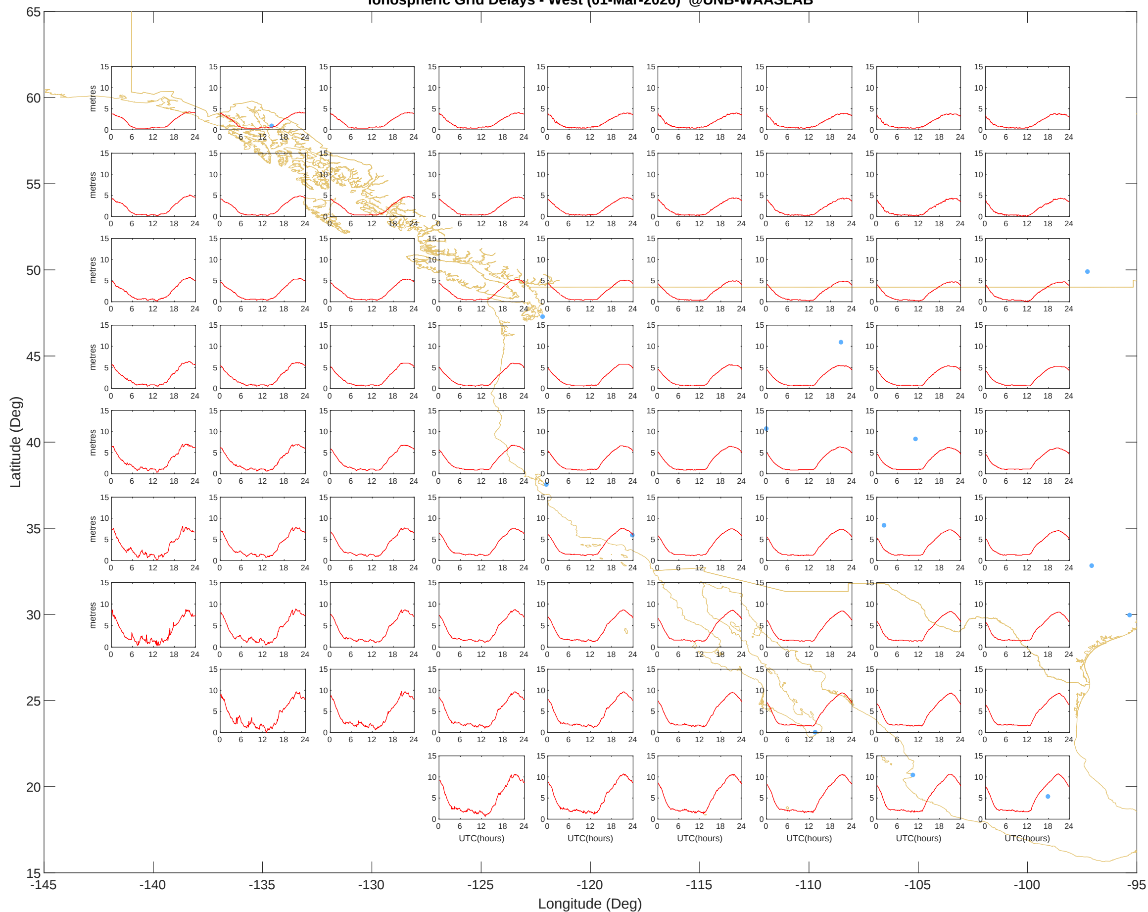
Ionospheric Grid Delays - West (01-Mar-2026) @UNB-WAASLAB
