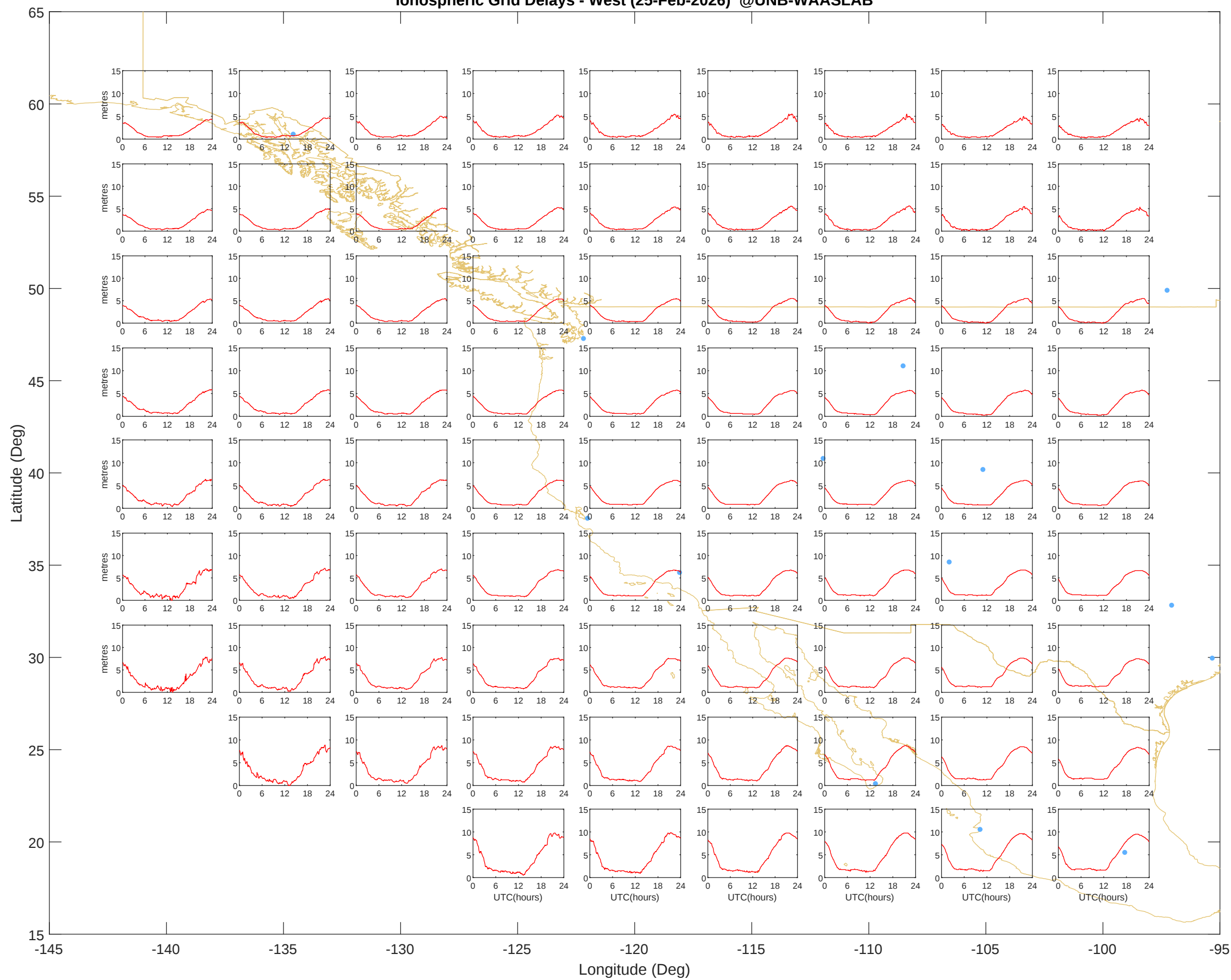
Ionospheric Grid Delays - West (25-Feb-2026) @UNB-WAASLAB
