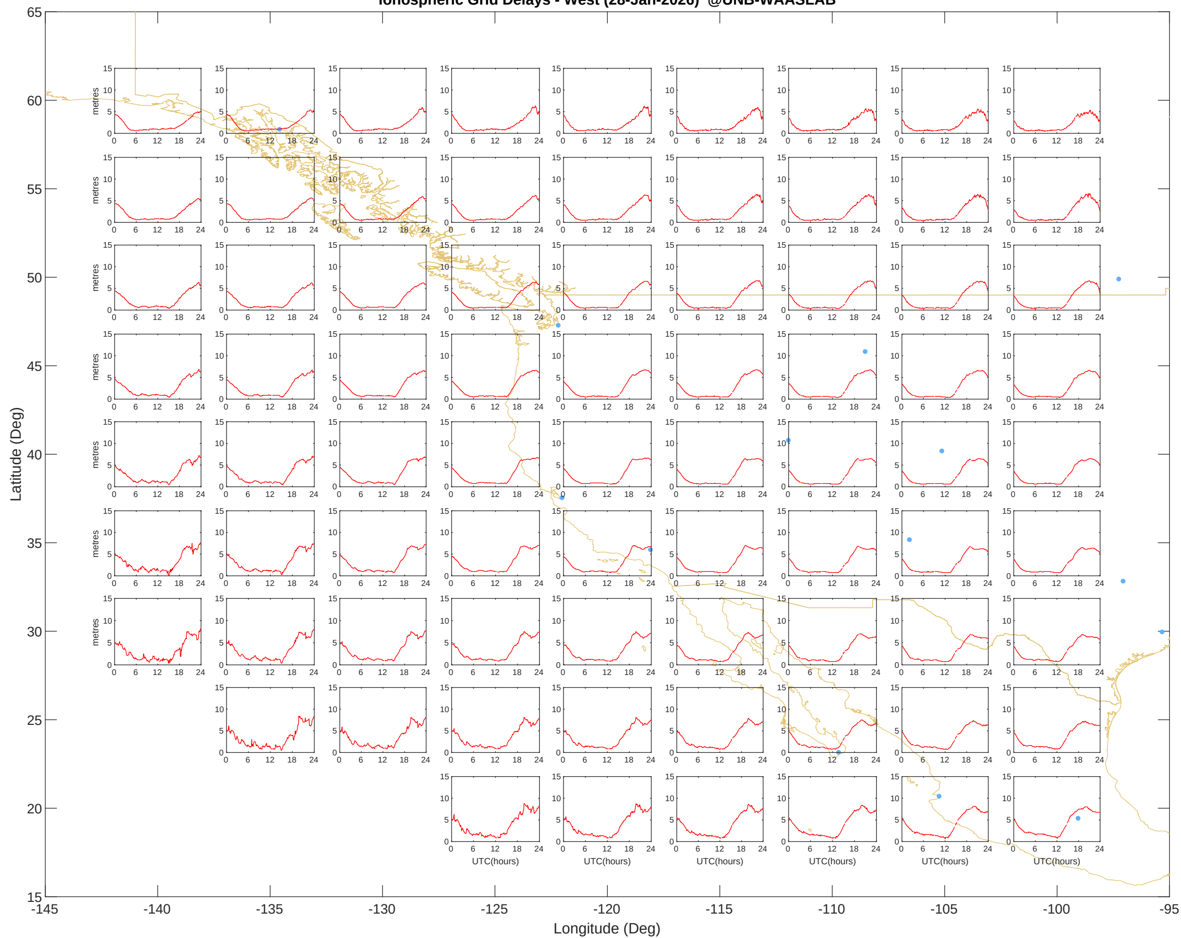
Ionospheric Grid Delays - West (28-Jan-2026) @UNB-WAASLAB
