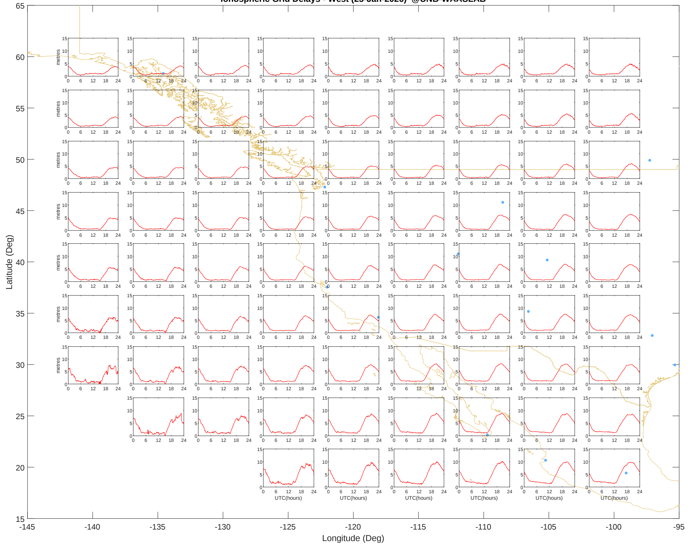
Ionospheric Grid Delays - West (25-Jan-2026) @UNB-WAASLAB
