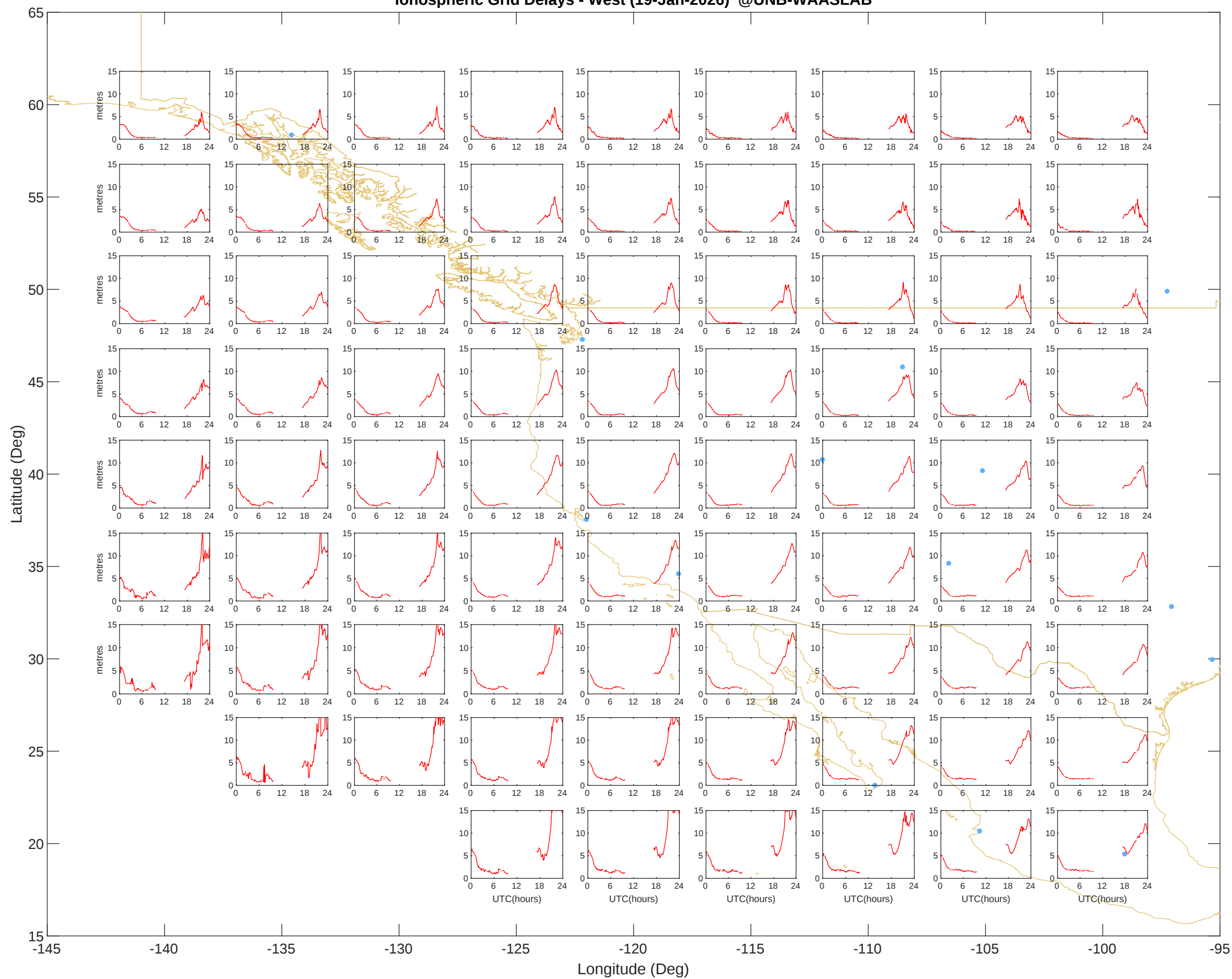
Ionospheric Grid Delays - West (19-Jan-2026) @UNB-WAASLAB
