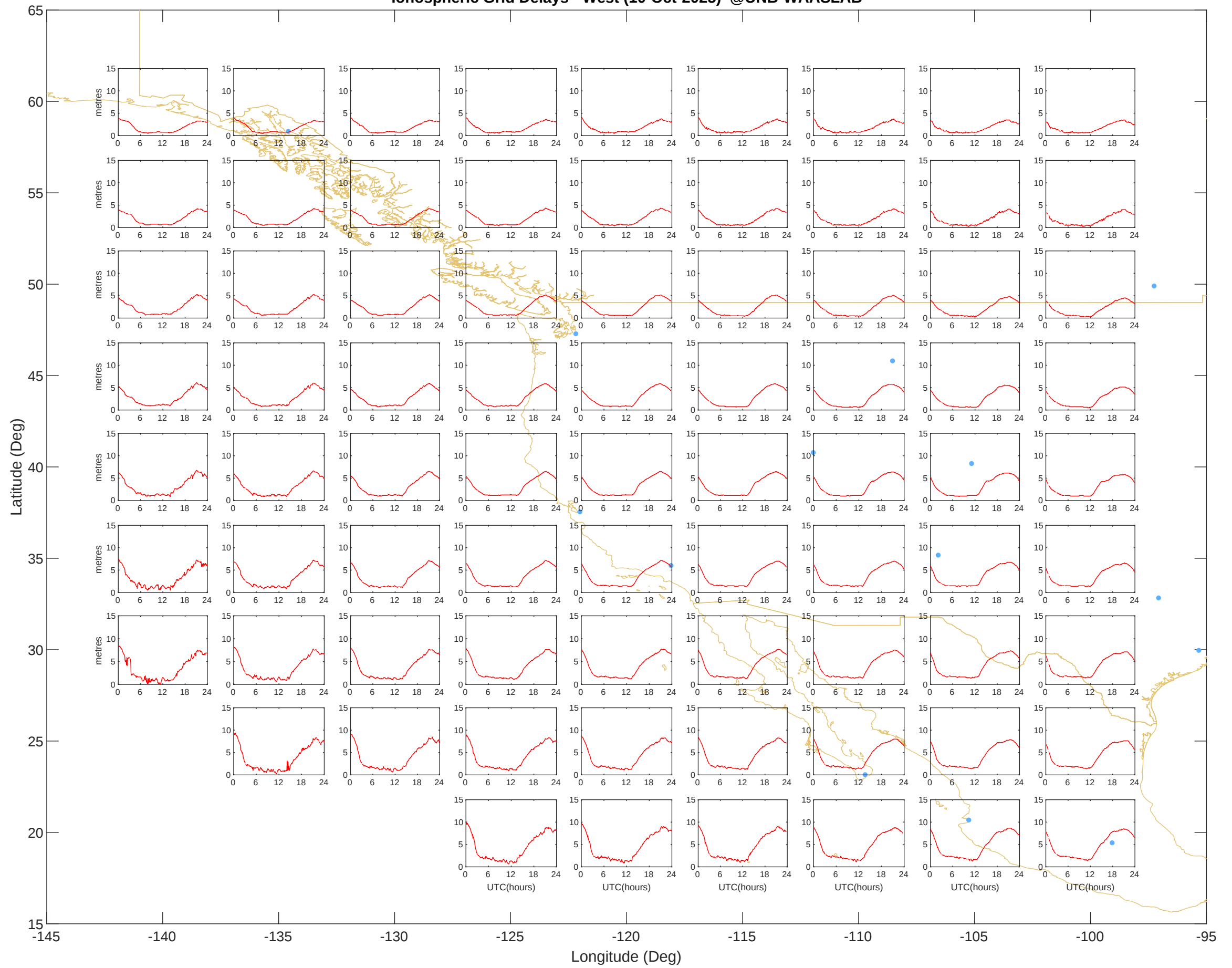
Ionospheric Grid Delays - West (10-Oct-2025) @UNB-WAASLAB
