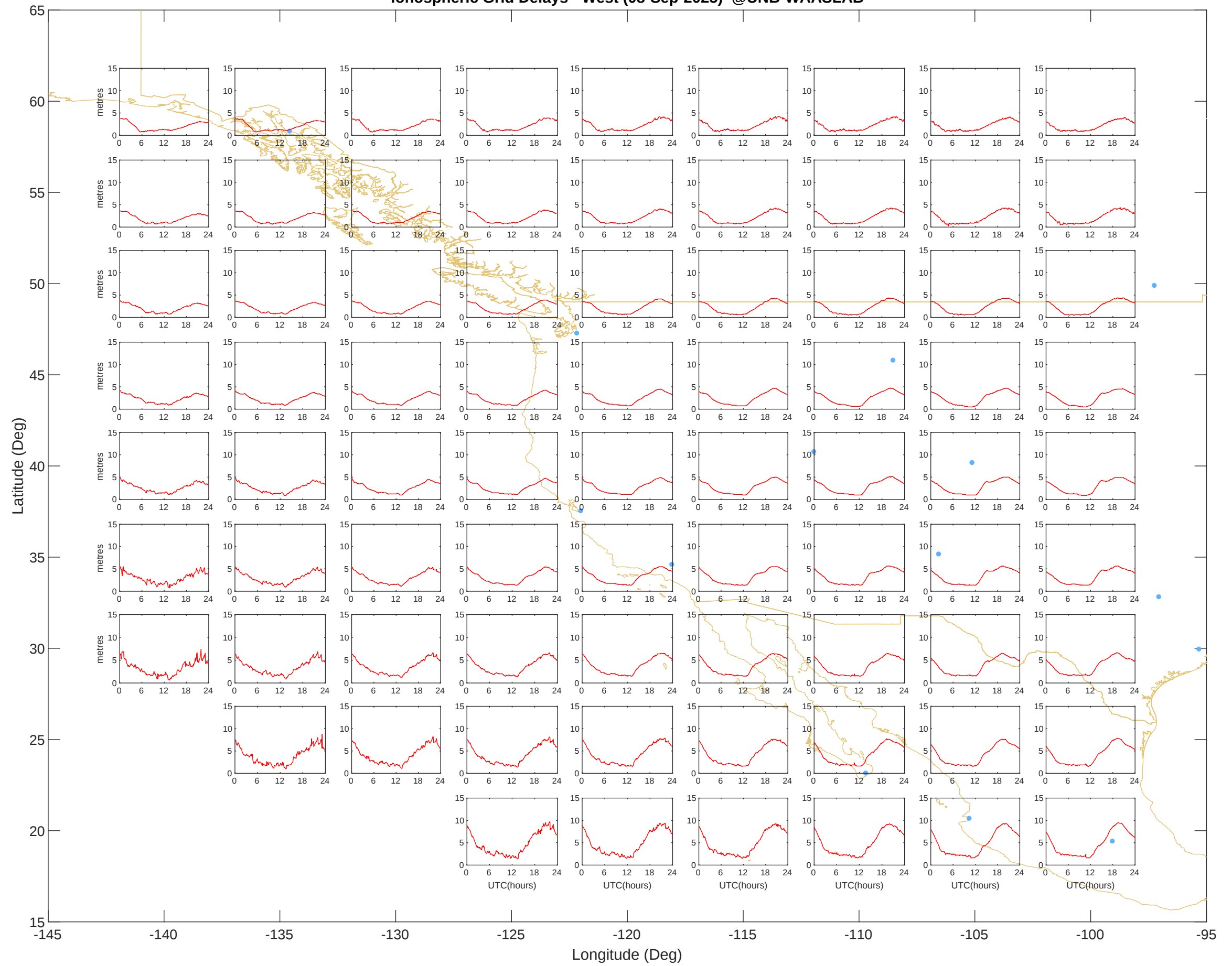
Ionospheric Grid Delays - West (08-Sep-2025) @UNB-WAASLAB
