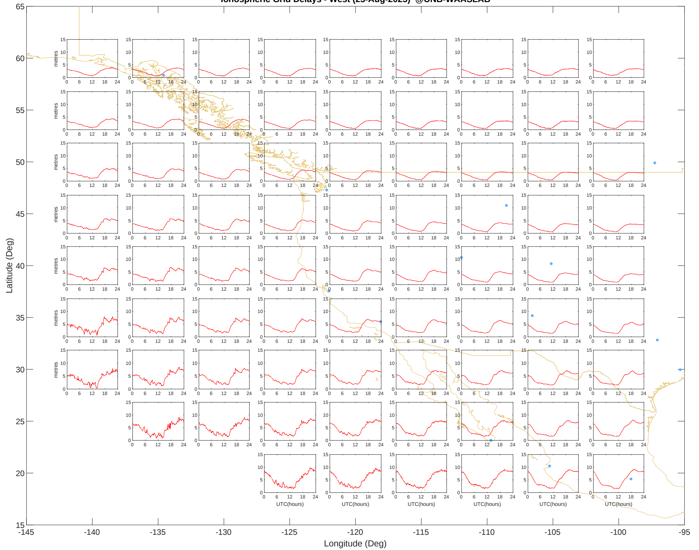
Ionospheric Grid Delays - West (25-Aug-2025) @UNB-WAASLAB
