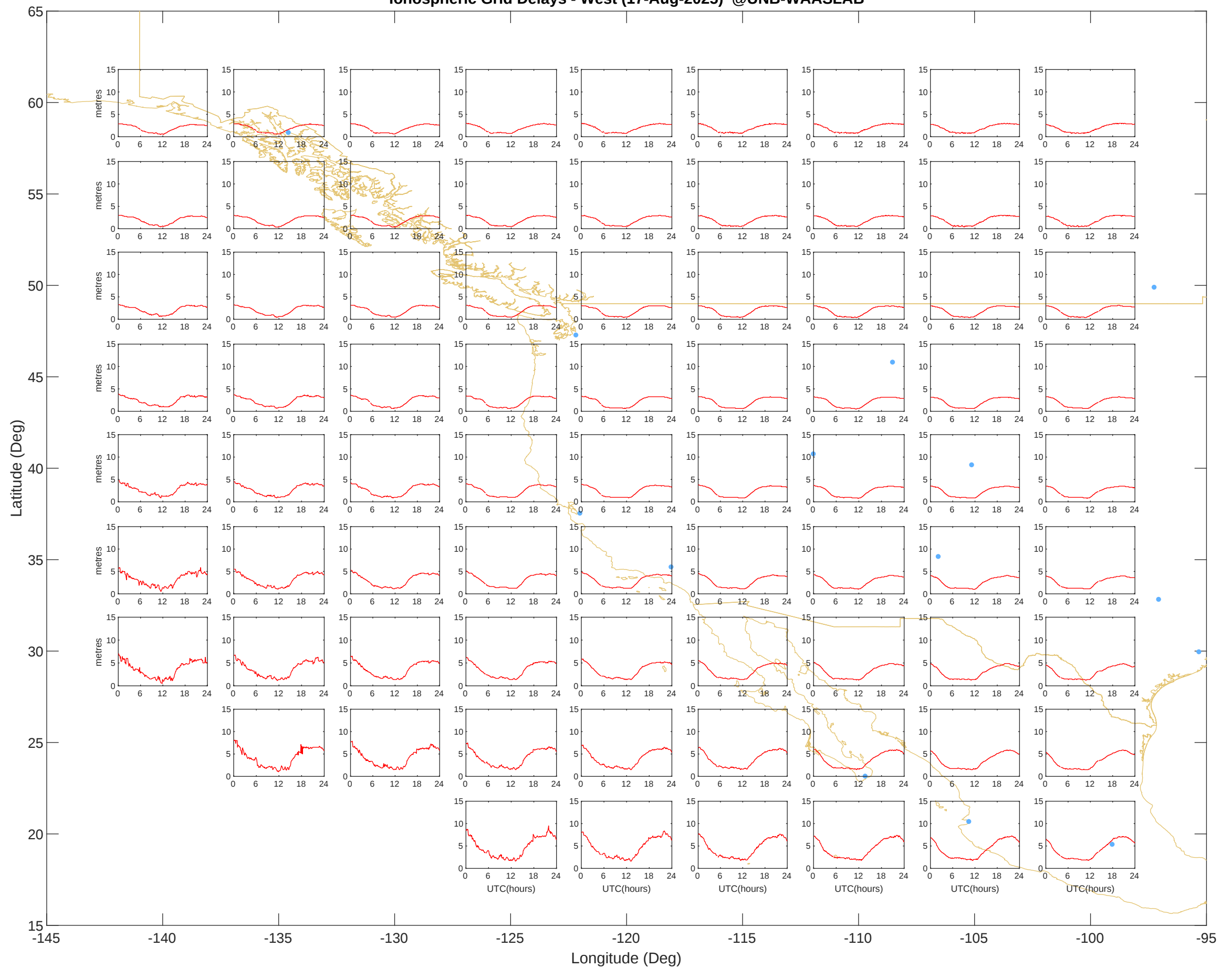
Ionospheric Grid Delays - West (17-Aug-2025) @UNB-WAASLAB
