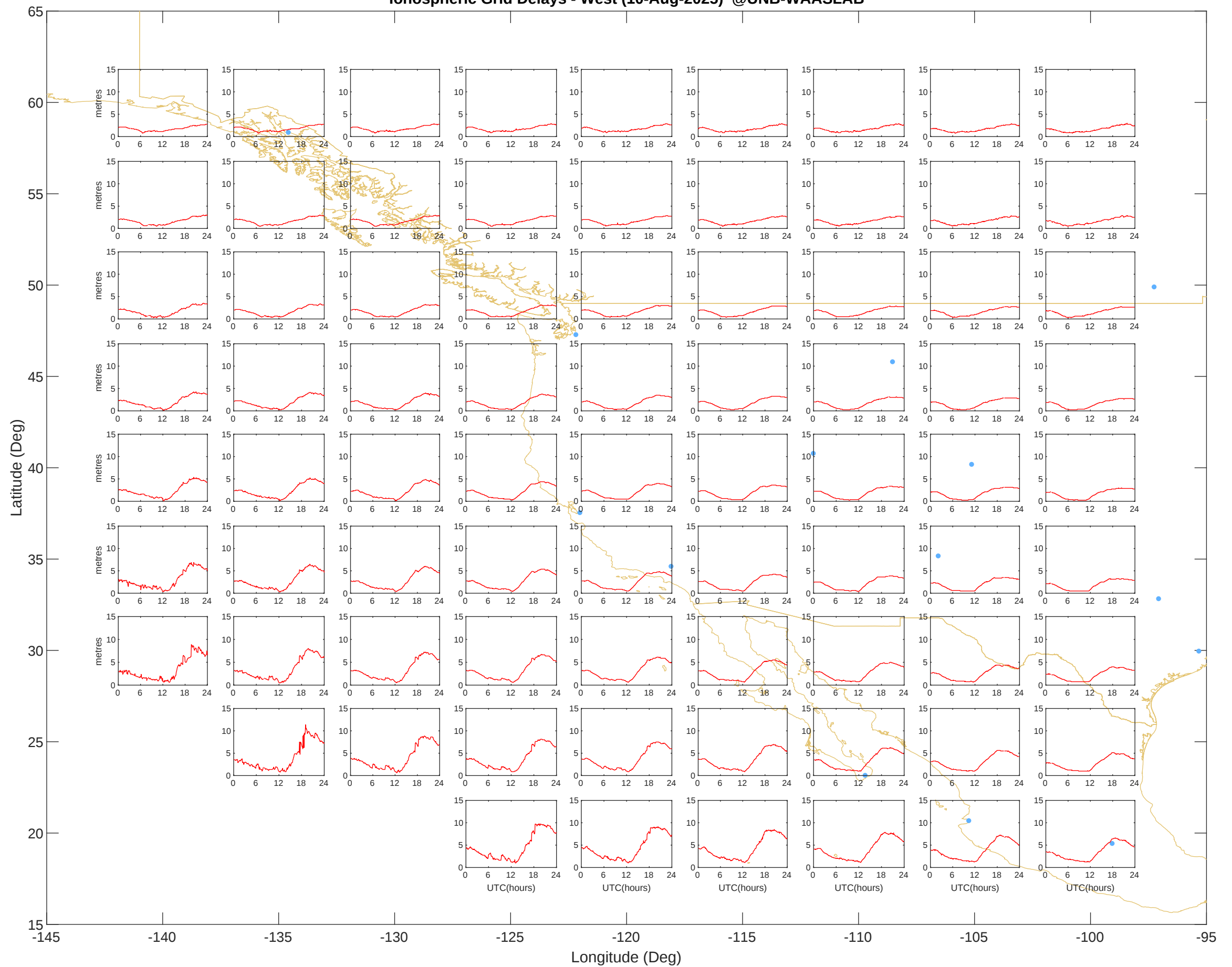
Ionospheric Grid Delays - West (10-Aug-2025) @UNB-WAASLAB
