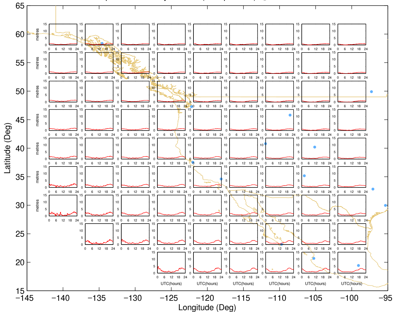
Ionospheric Grid Delays – West (01-Apr-2019) @UNB-WAASLAB
