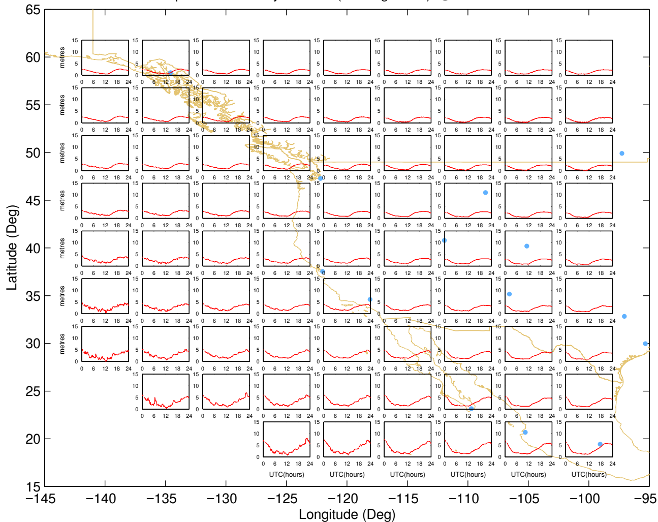
Ionospheric Grid Delays – West (31-Aug-2011) @UNB-WAASLAB
