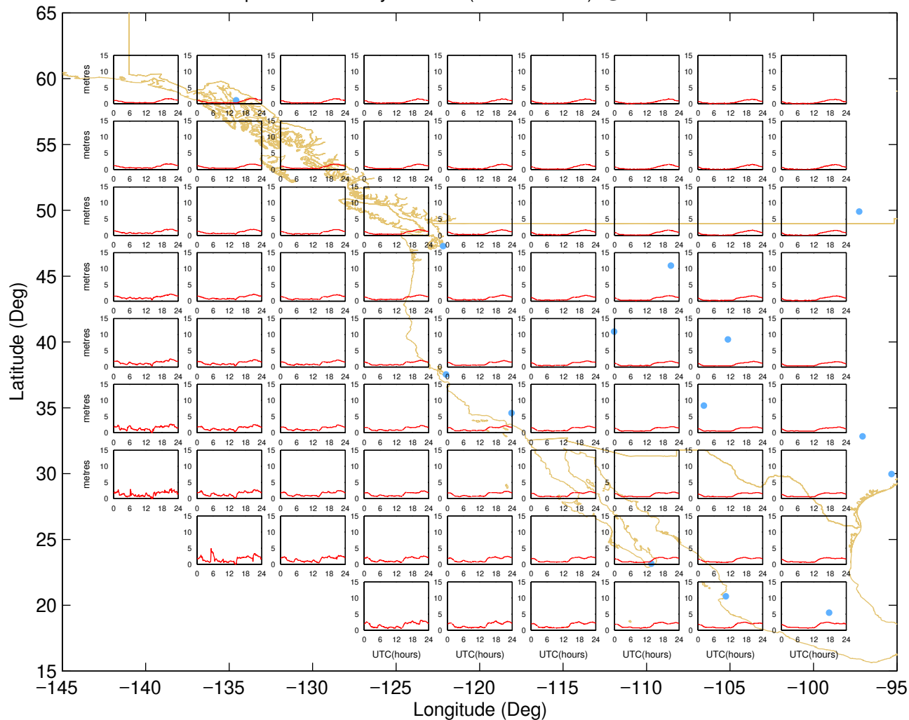
Ionospheric Grid Delays – West (13-Oct-2009) @UNB-WAASLAB
