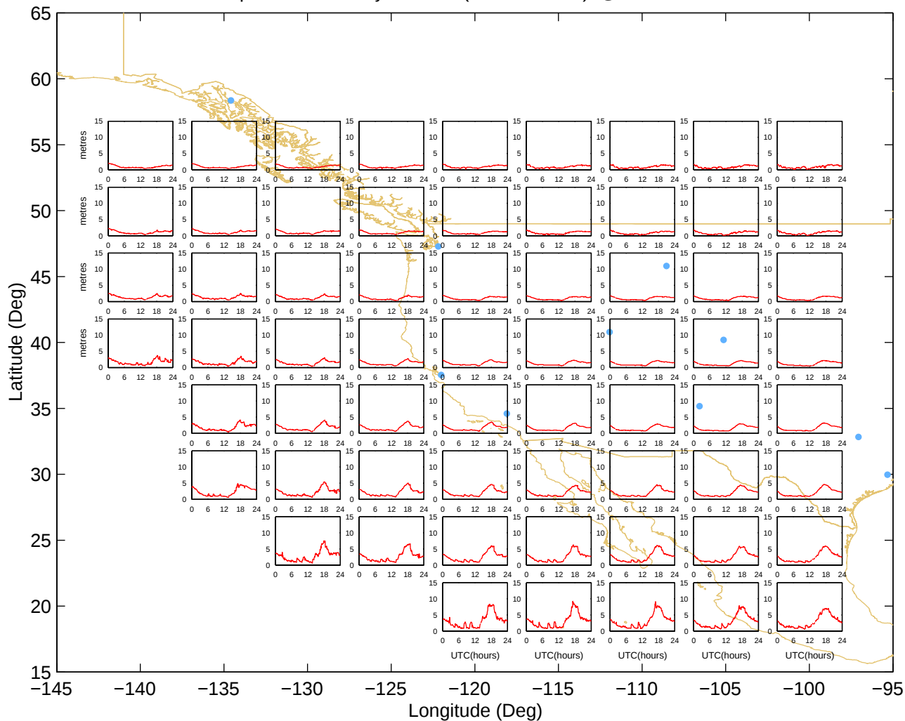
Ionospheric Grid Delays – West (13-Oct-2004) @UNB-WAASLAB
