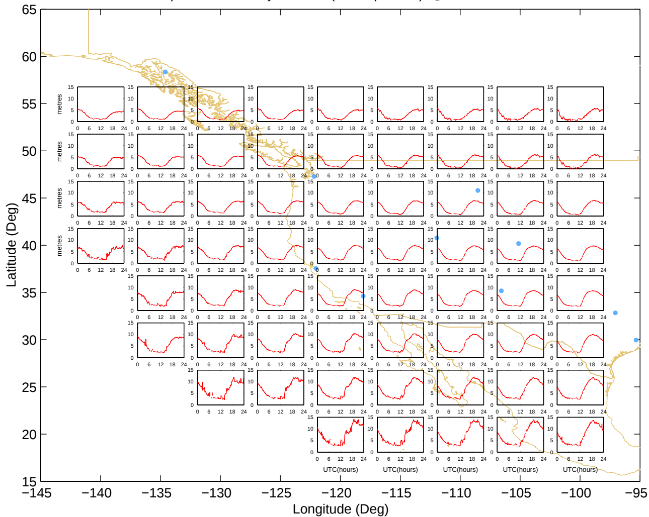
Ionospheric Grid Delays – West (13-Sep-2002) @UNB-WAASLAB
