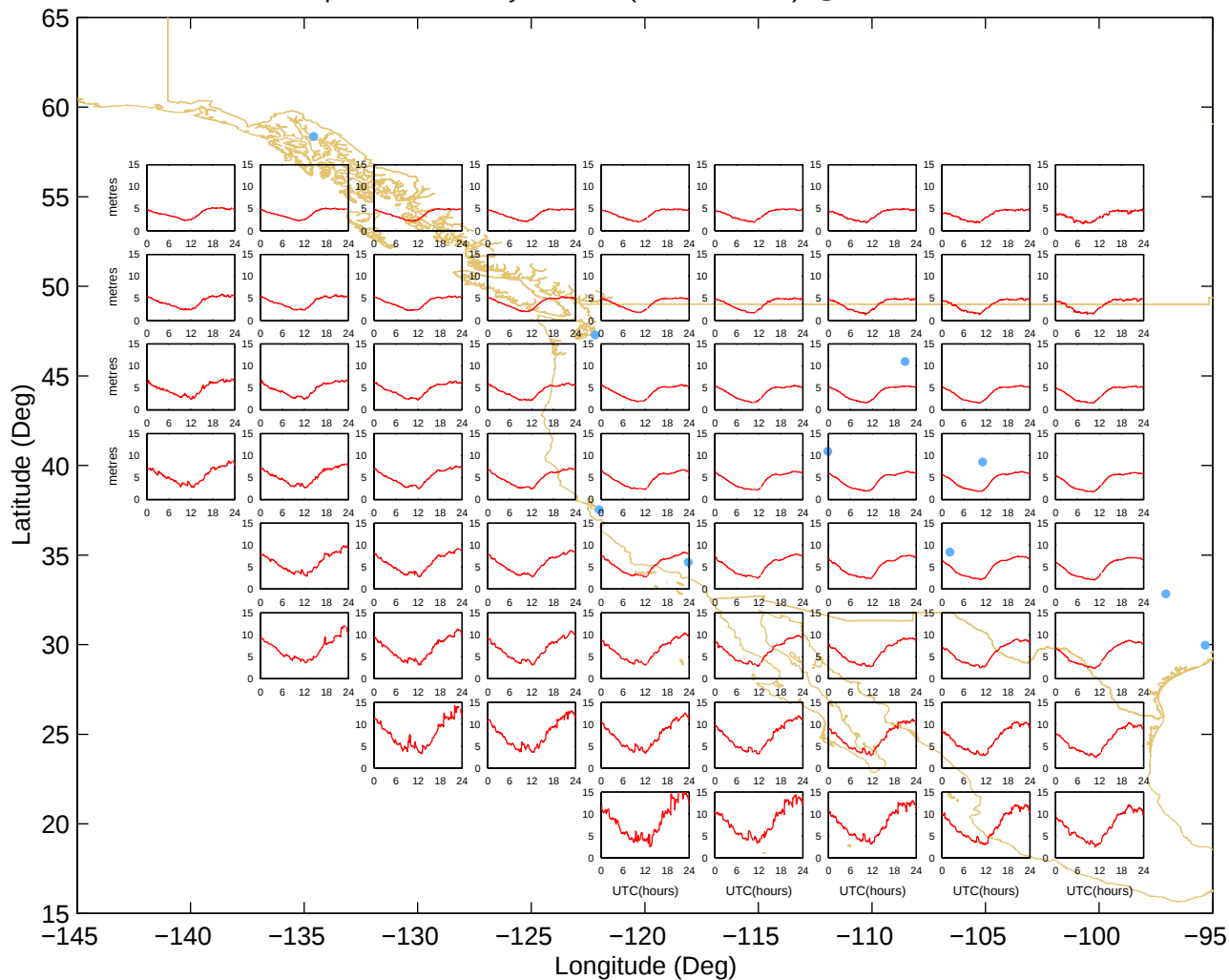
Ionospheric Grid Delays – West (01-Jun-2002) @UNB-WAASLAB
