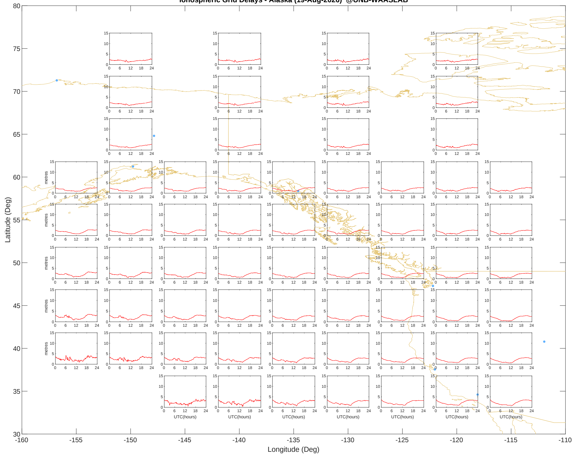
Ionospheric Grid Delays - Alaska (19-Aug-2026) @UNB-WAASLAB
