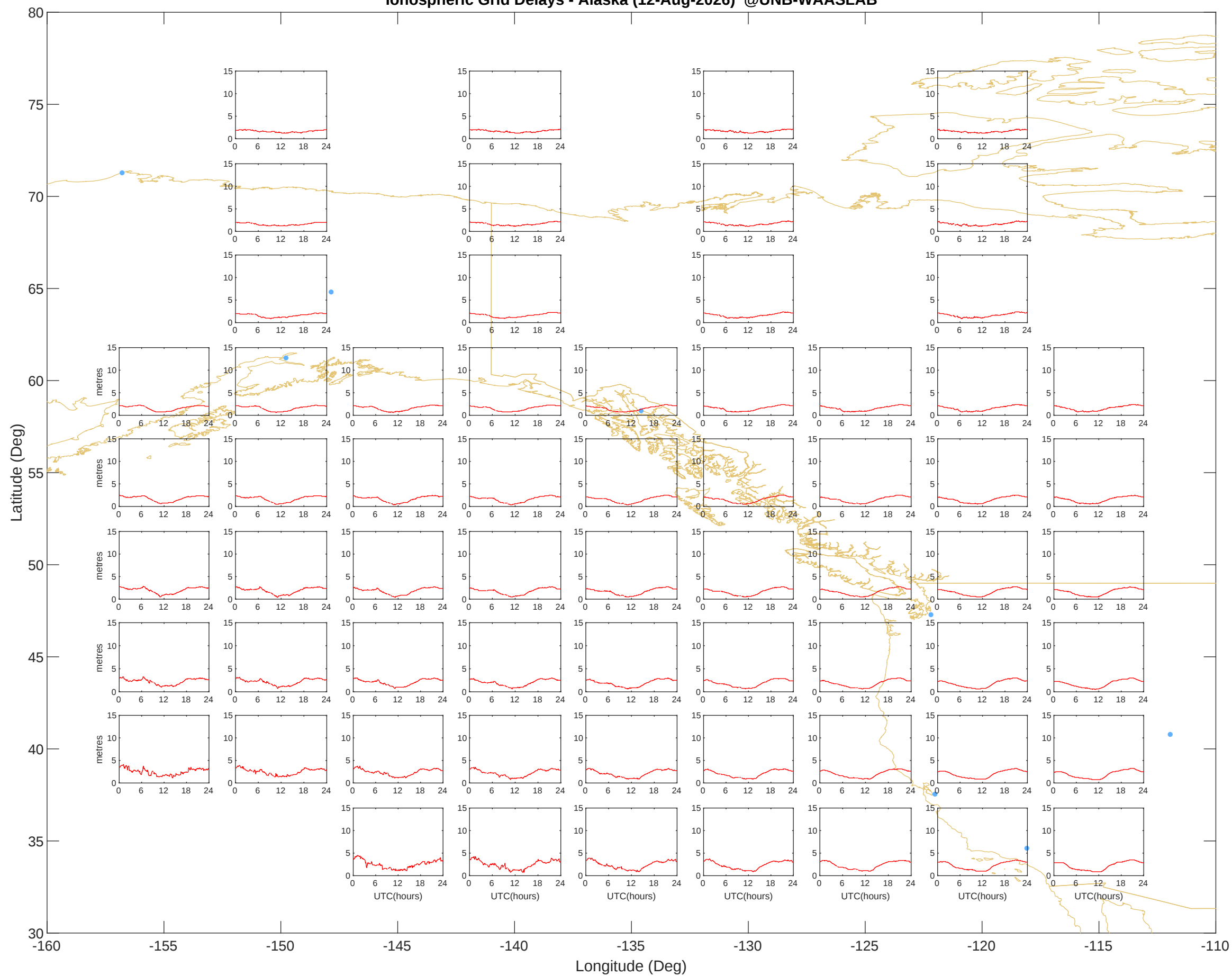
Ionospheric Grid Delays - Alaska (12-Aug-2026) @UNB-WAASLAB
