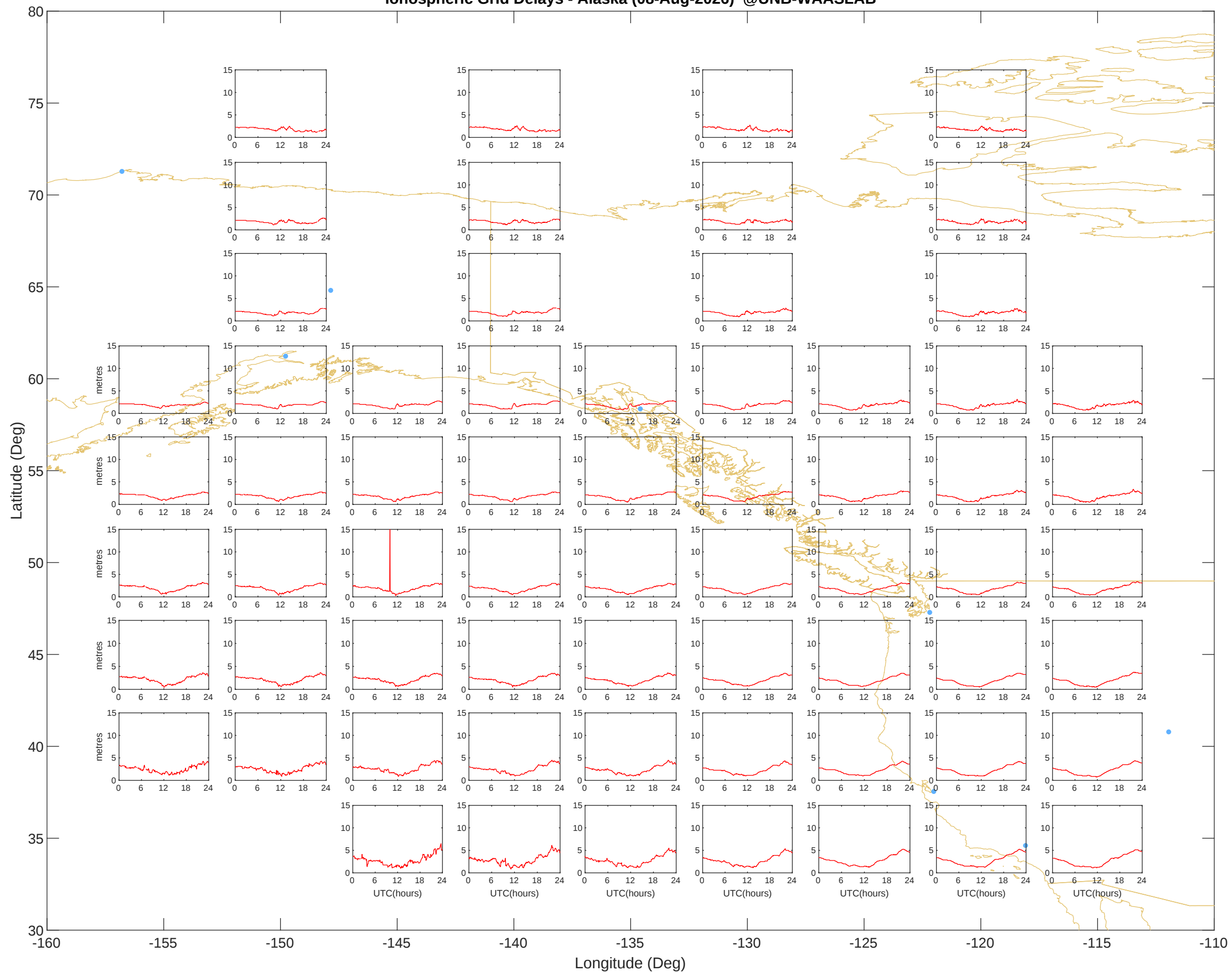
Ionospheric Grid Delays - Alaska (08-Aug-2026) @UNB-WAASLAB
