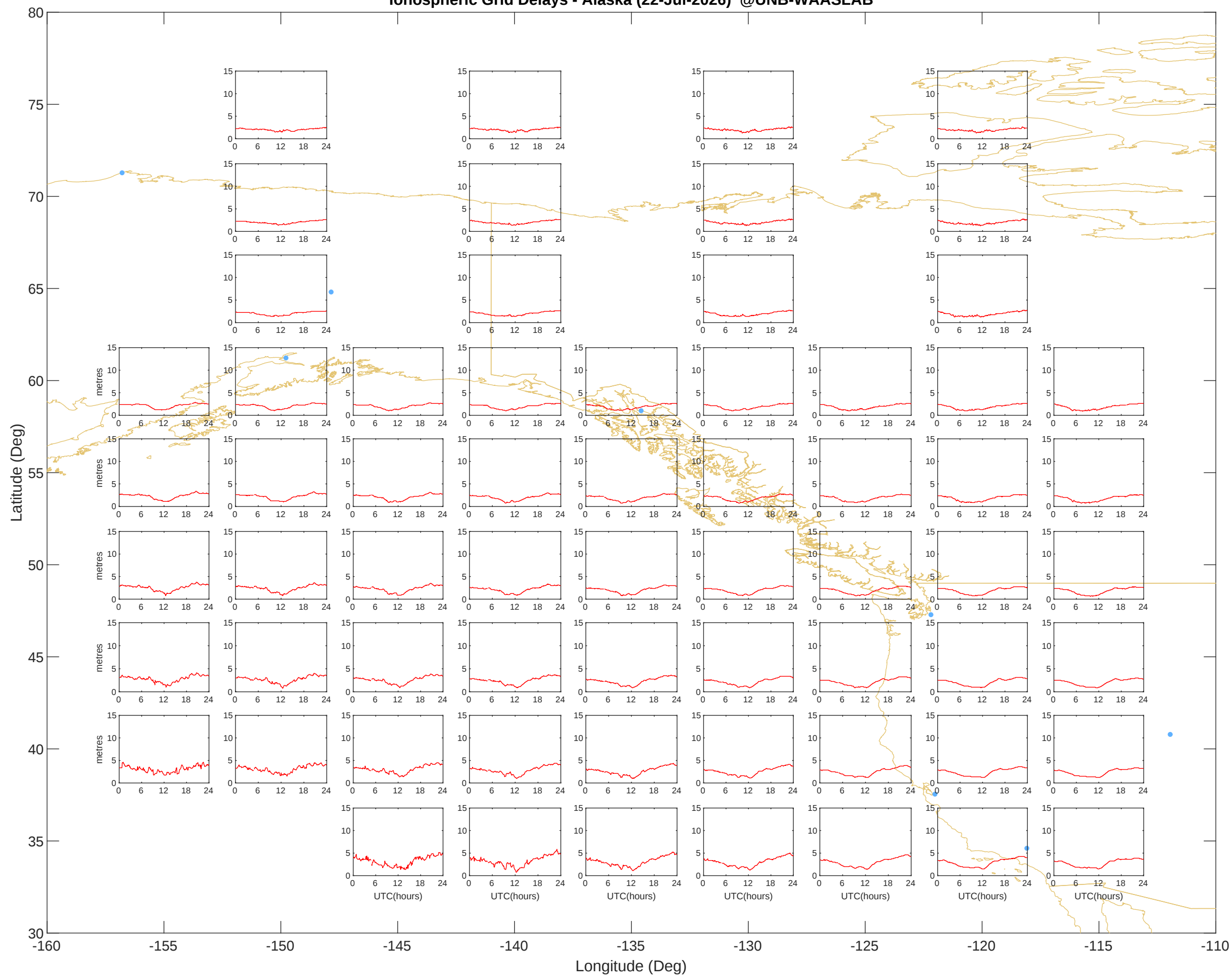
Ionospheric Grid Delays - Alaska (22-Jul-2026) @UNB-WAASLAB
