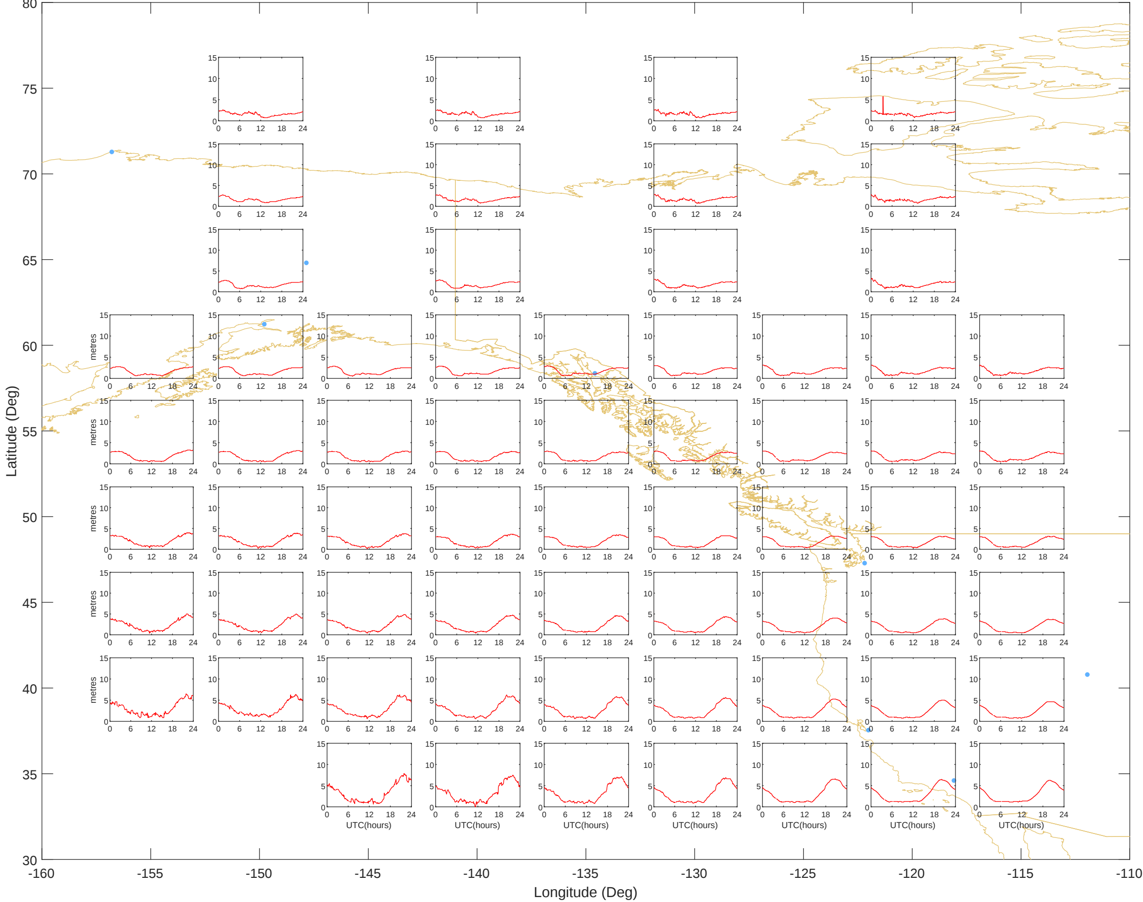
Ionospheric Grid Delays - Alaska (25-Mar-2026) @UNB-WAASLAB
