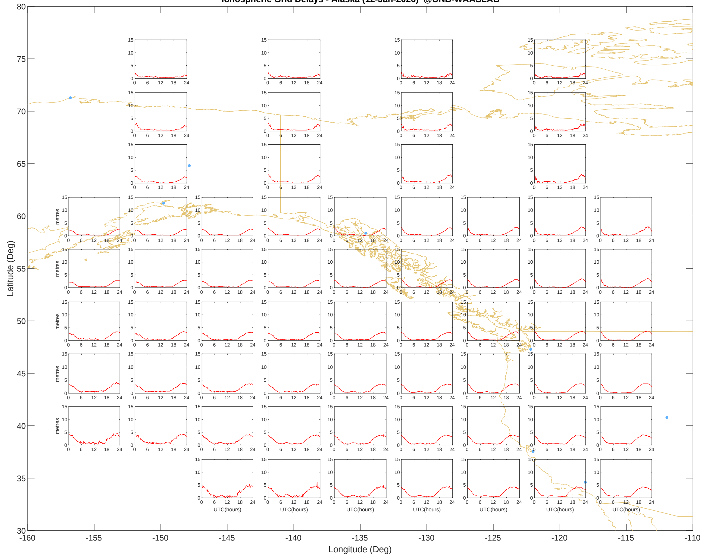
Ionospheric Grid Delays - Alaska (12-Jan-2026) @UNB-WAASLAB
