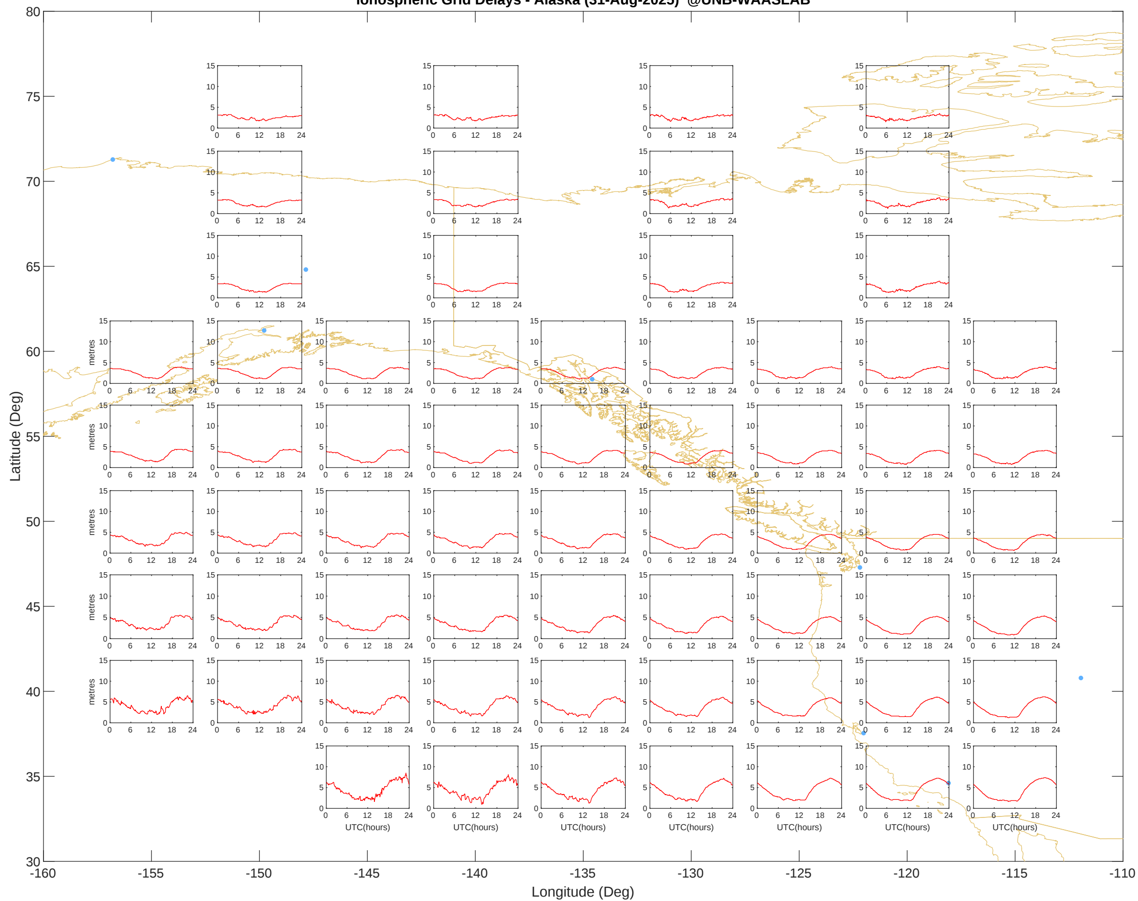
Ionospheric Grid Delays - Alaska (31-Aug-2025) @UNB-WAASLAB
