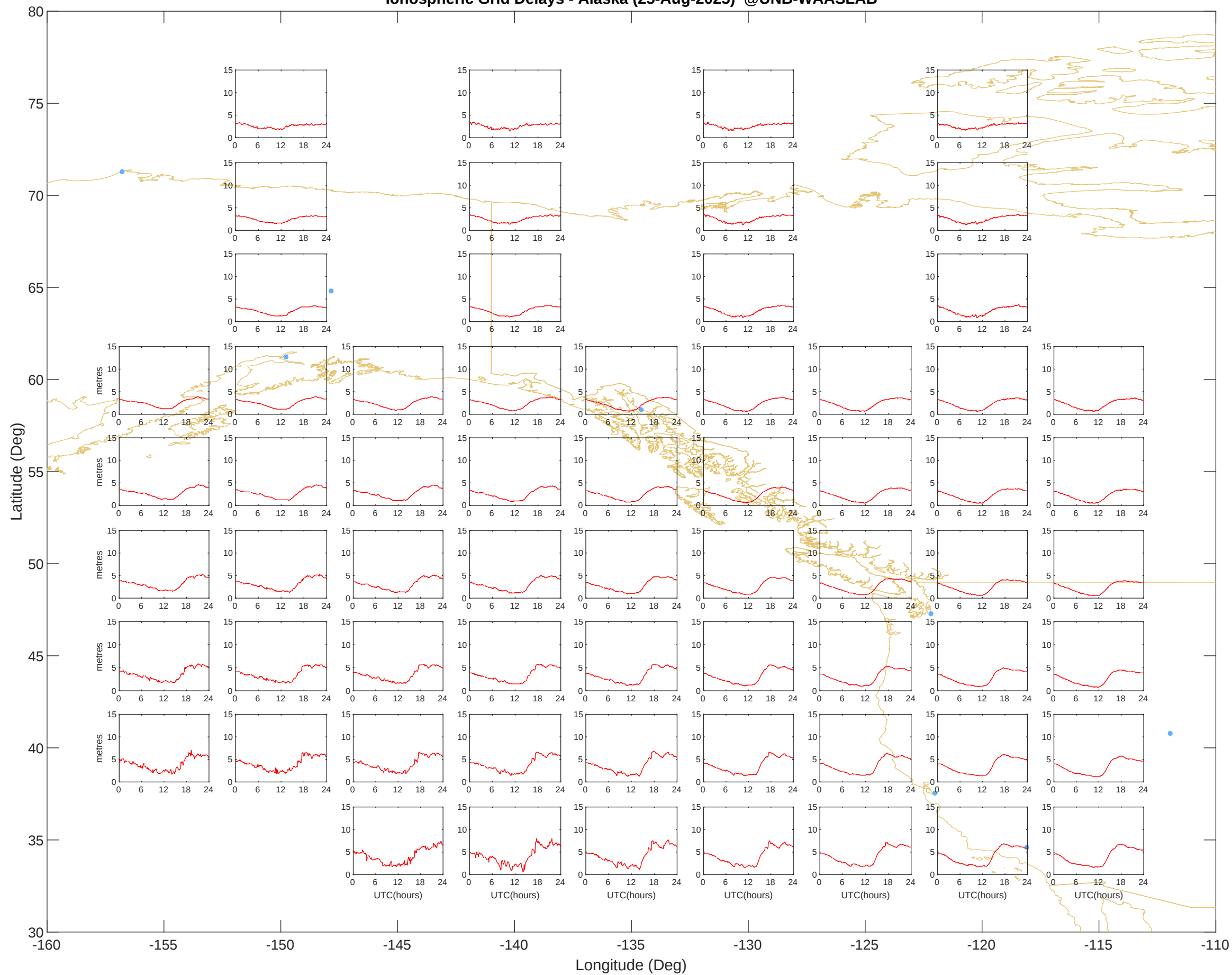
Ionospheric Grid Delays - Alaska (25-Aug-2025) @UNB-WAASLAB
