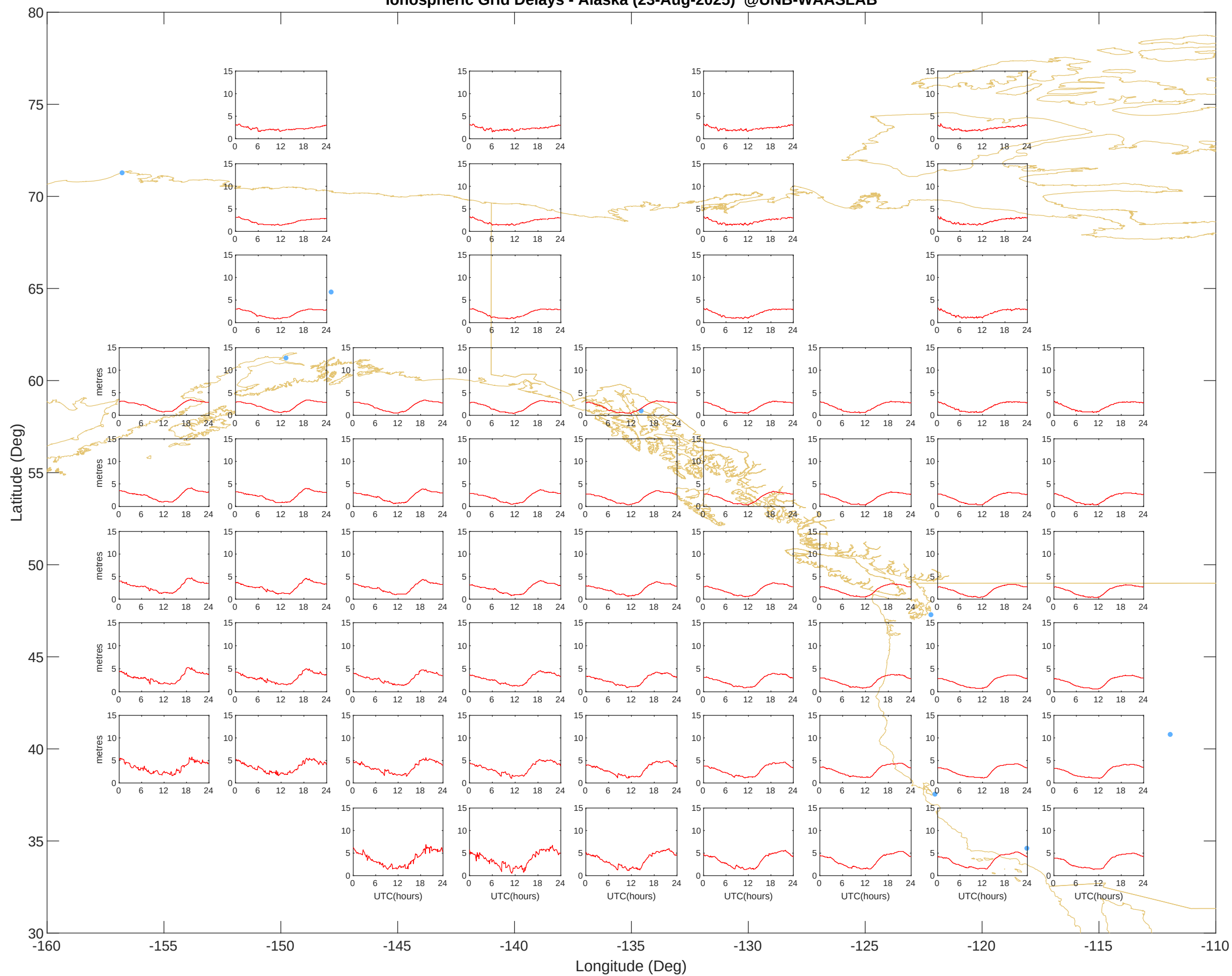
Ionospheric Grid Delays - Alaska (23-Aug-2025) @UNB-WAASLAB
