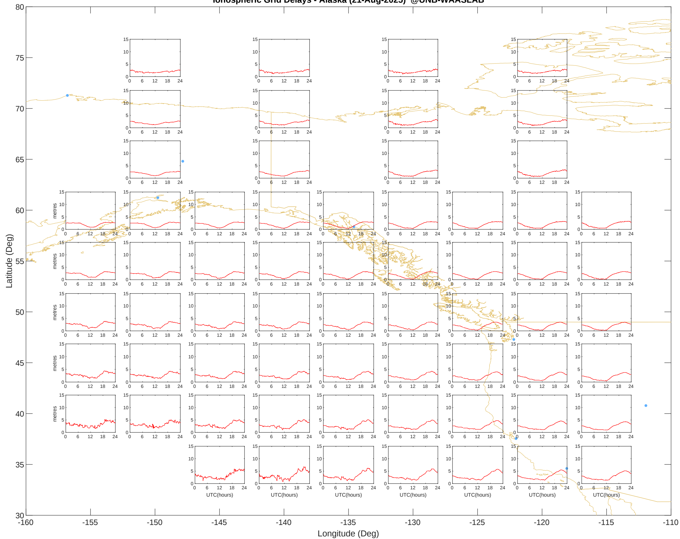
Ionospheric Grid Delays - Alaska (21-Aug-2025) @UNB-WAASLAB
