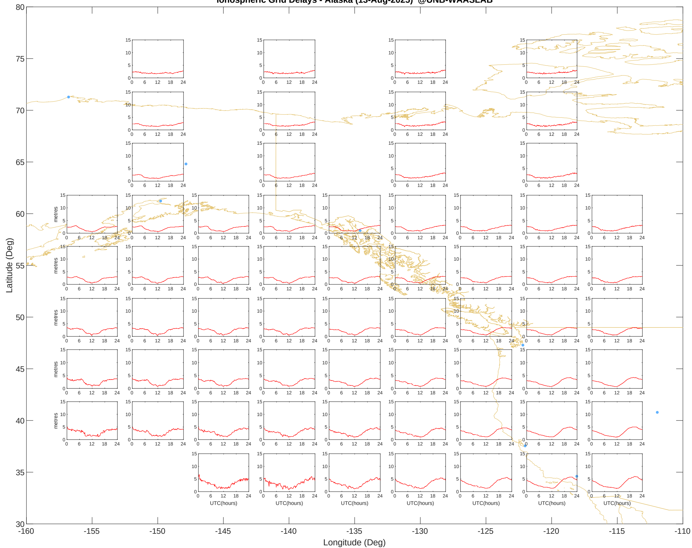
Ionospheric Grid Delays - Alaska (13-Aug-2025) @UNB-WAASLAB
