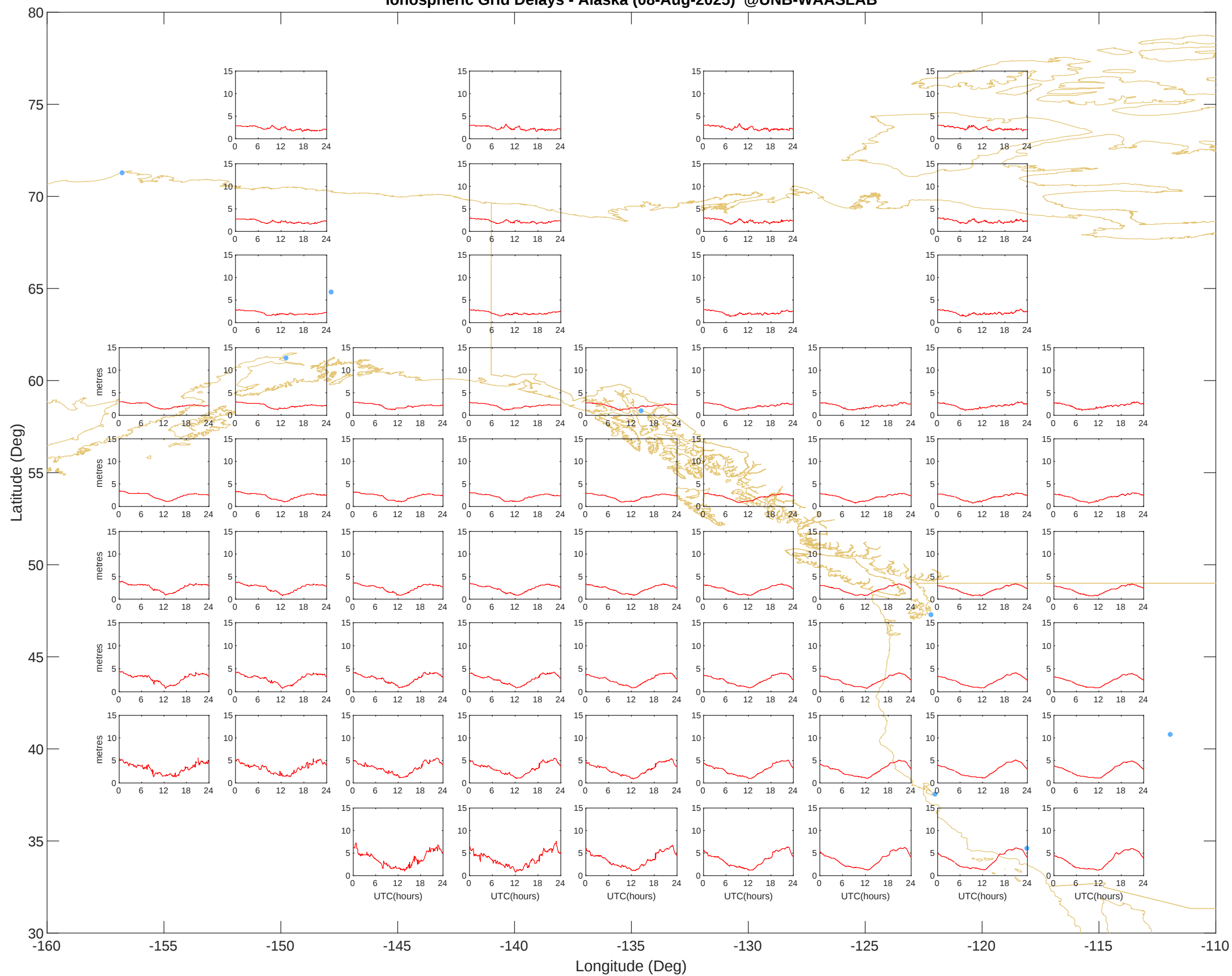
Ionospheric Grid Delays - Alaska (08-Aug-2025) @UNB-WAASLAB
