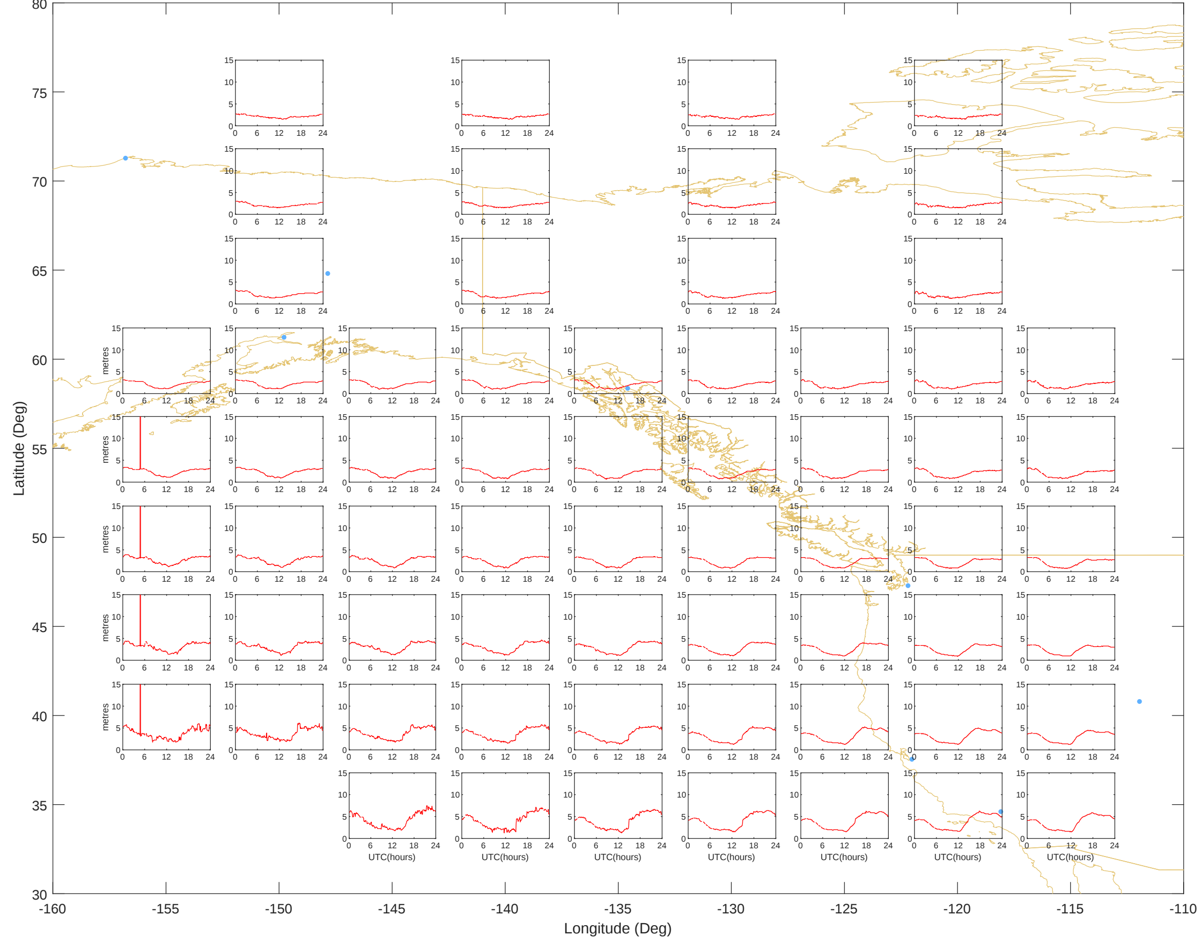
Ionospheric Grid Delays - Alaska (21-May-2025) @UNB-WAASLAB
