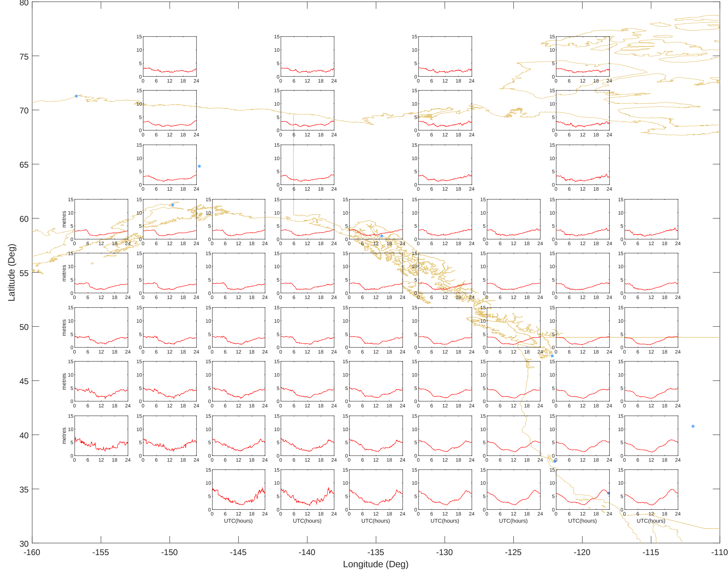
Ionospheric Grid Delays - Alaska (01-May-2025) @UNB-WAASLAB
