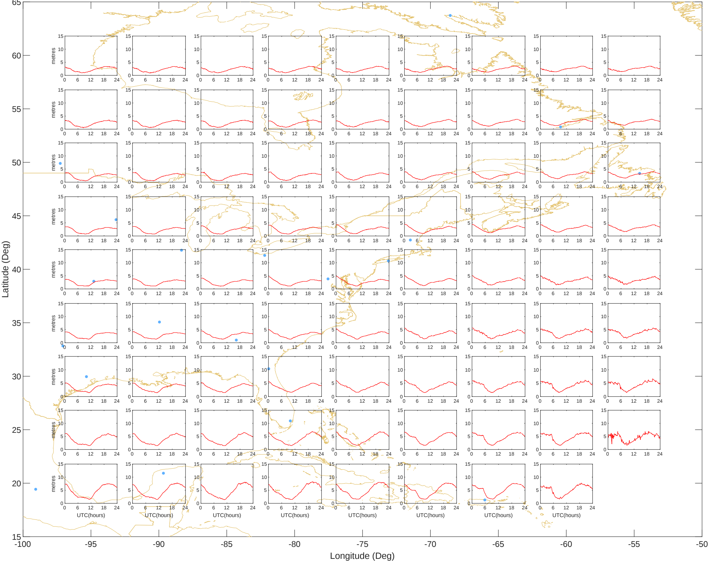
Ionospheric Grid Delays - East (28-Jul-2026) @UNB-WAASLAB
