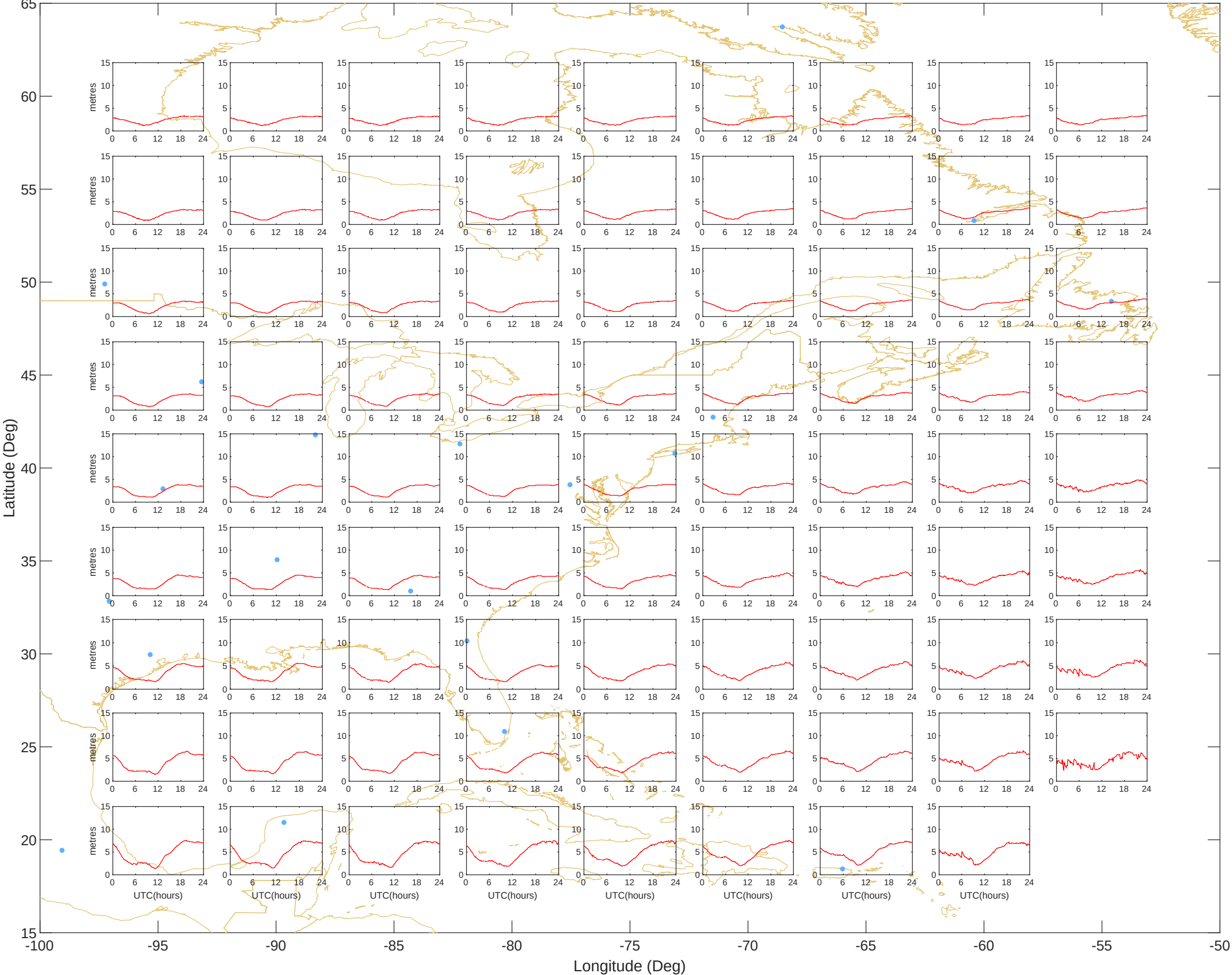
Ionospheric Grid Delays - East (26-Jul-2026) @UNB-WAASLAB
