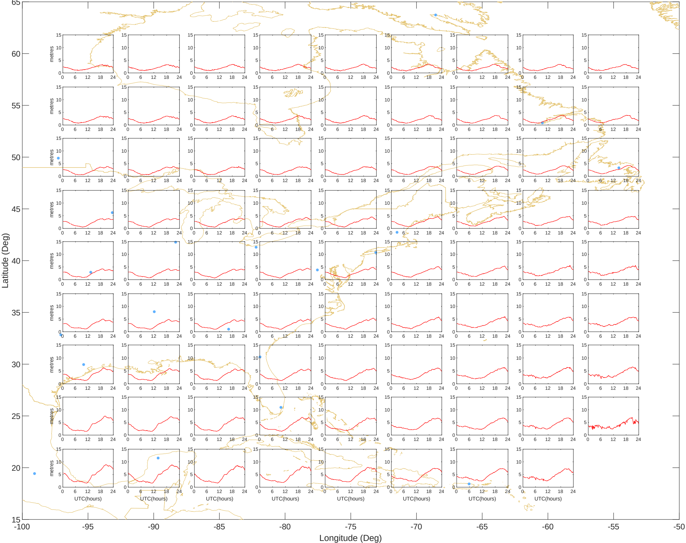
Ionospheric Grid Delays - East (23-Jul-2026) @UNB-WAASLAB
