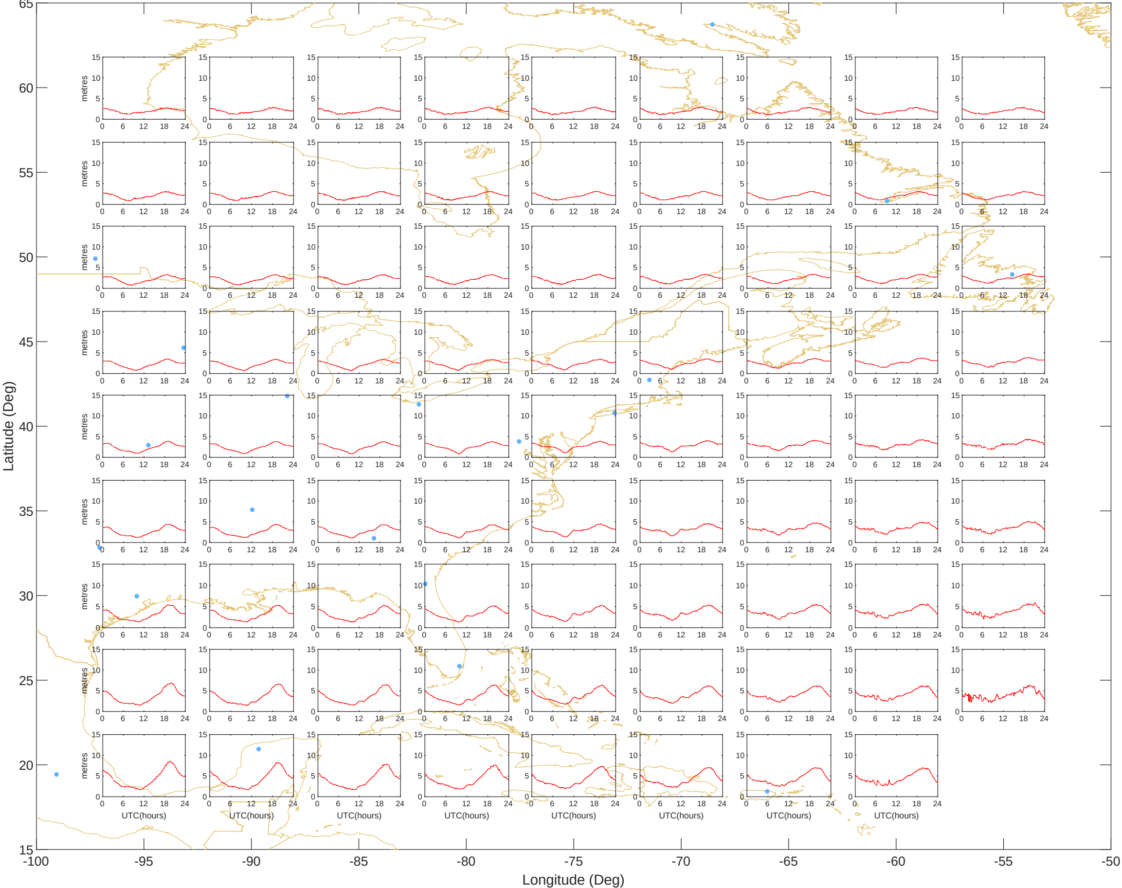
Ionospheric Grid Delays - East (21-Jul-2026) @UNB-WAASLAB
