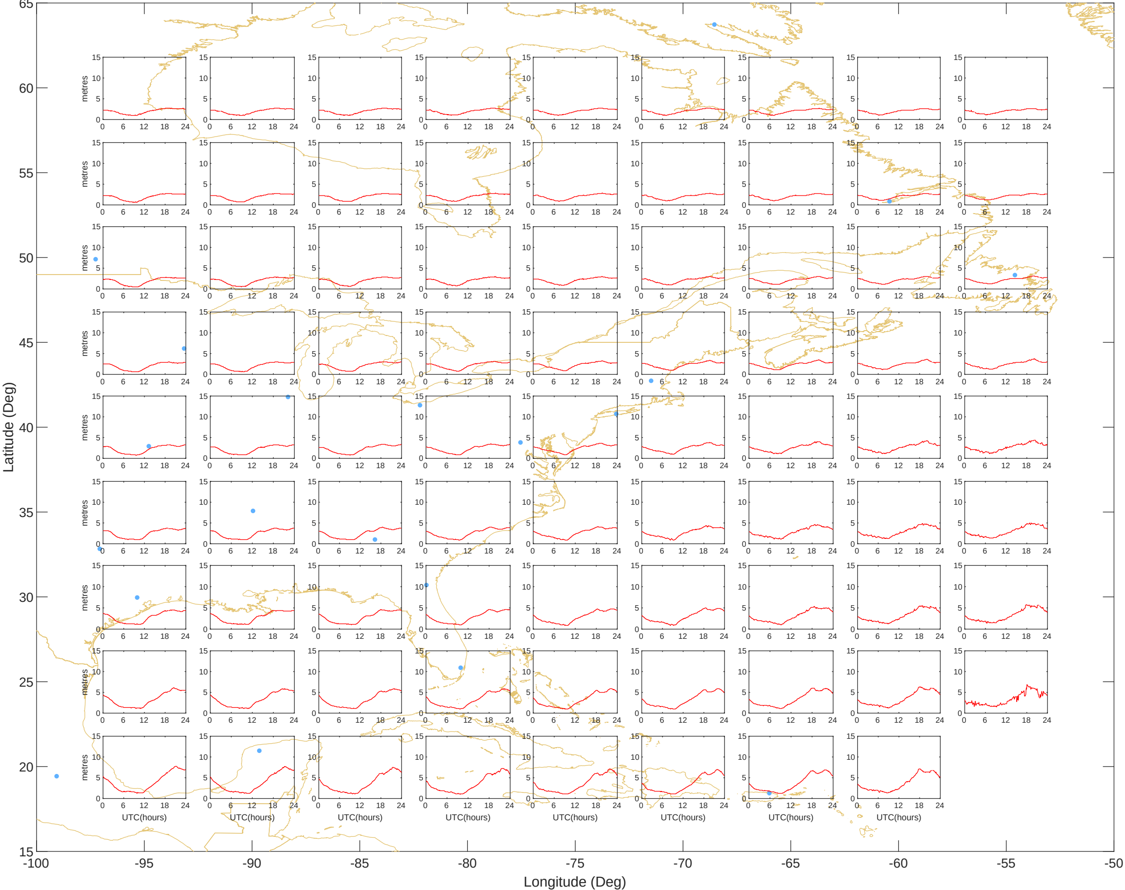
Ionospheric Grid Delays - East (19-Jul-2026) @UNB-WAASLAB
