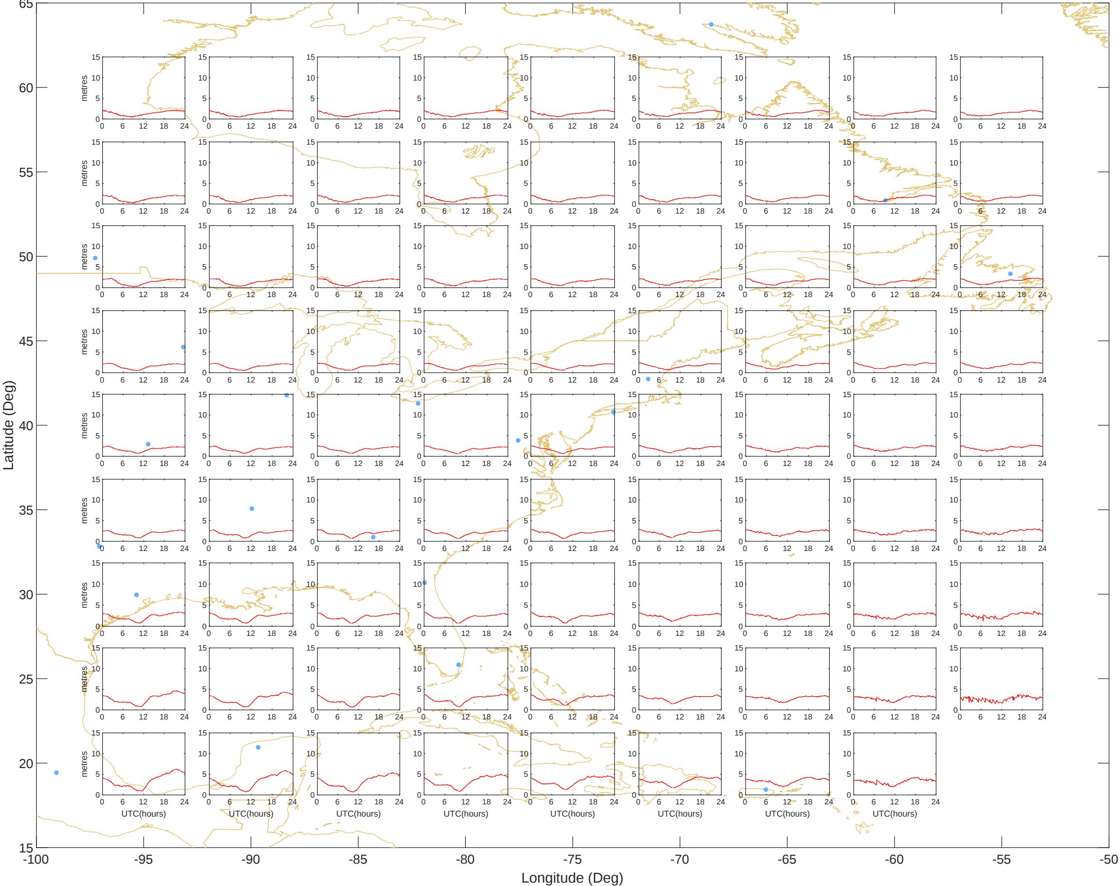
Ionospheric Grid Delays - East (16-Jul-2026) @UNB-WAASLAB
