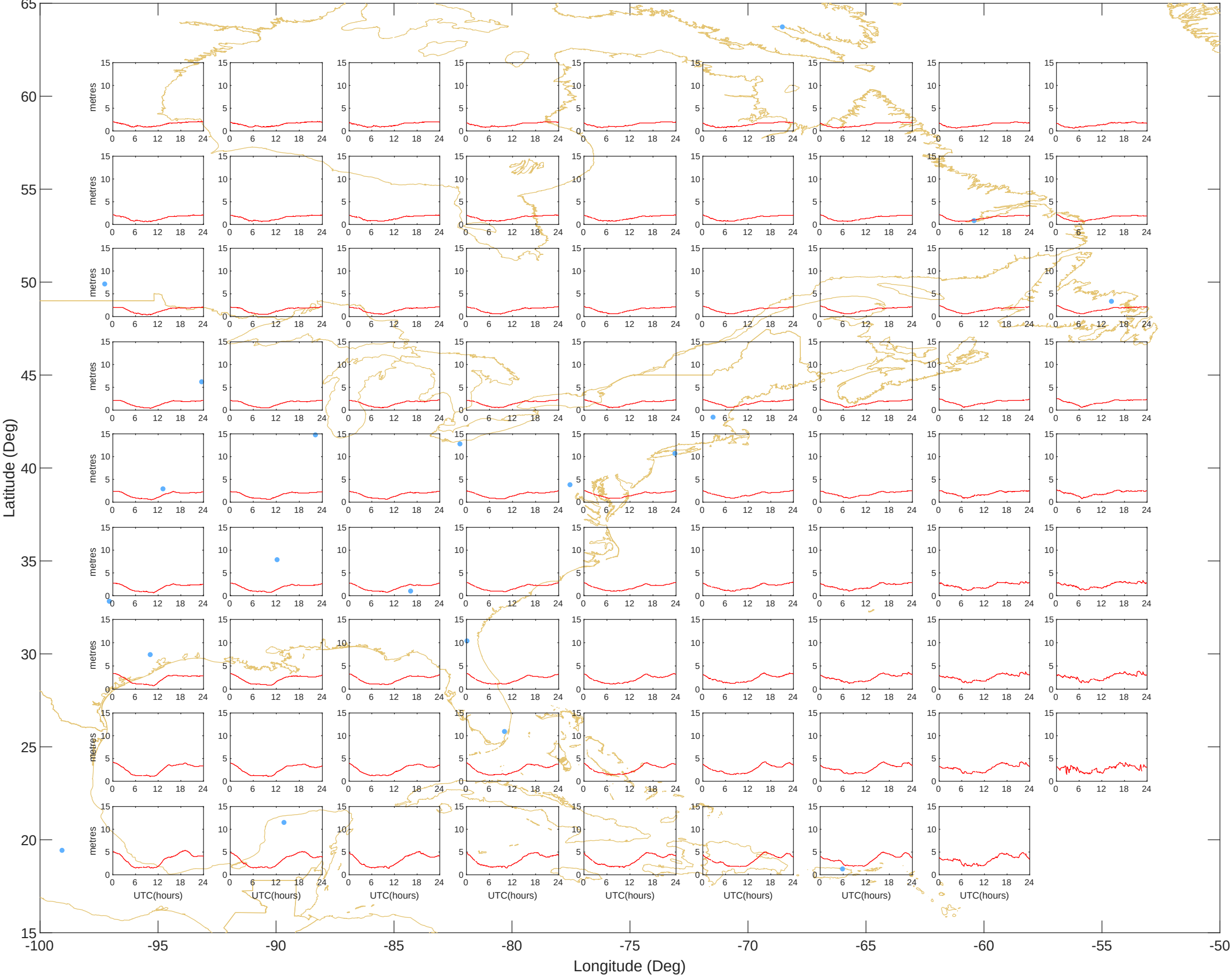
Ionospheric Grid Delays - East (15-Jul-2026) @UNB-WAASLAB
