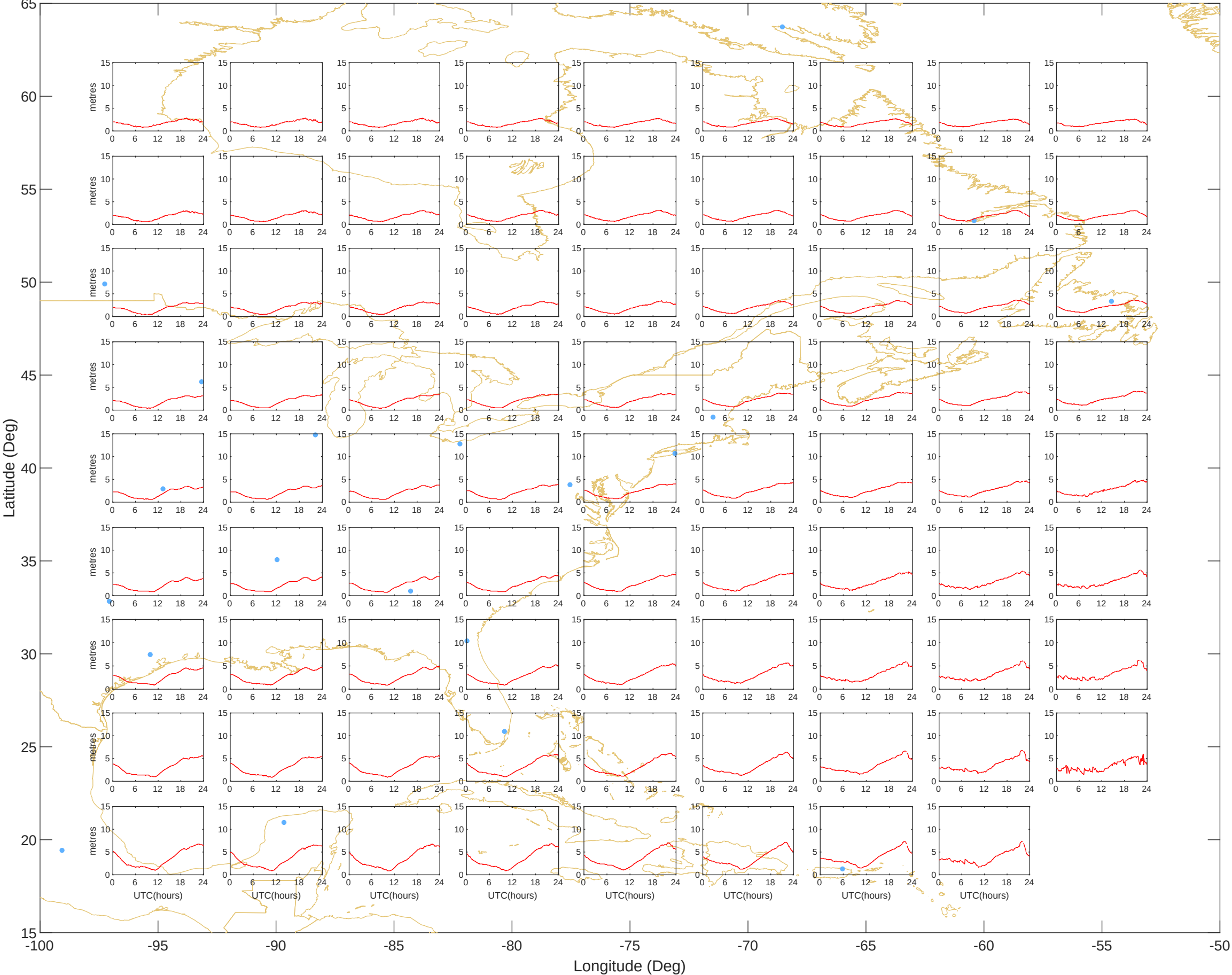
Ionospheric Grid Delays - East (13-Jul-2026) @UNB-WAASLAB
