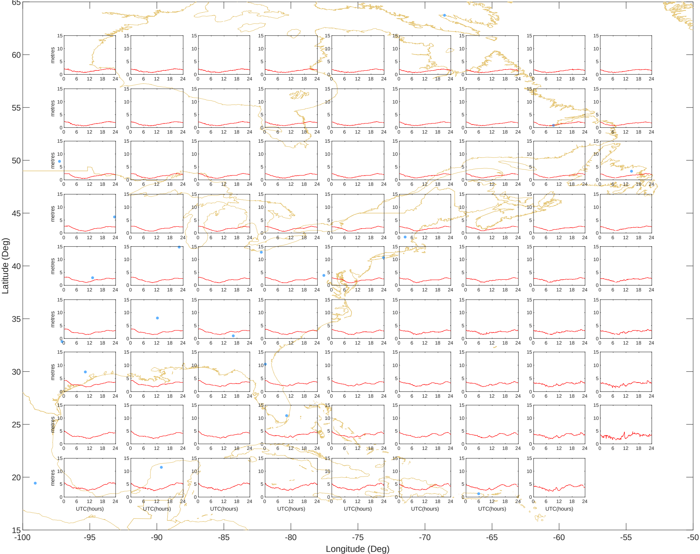
Ionospheric Grid Delays - East (08-Jul-2026) @UNB-WAASLAB
