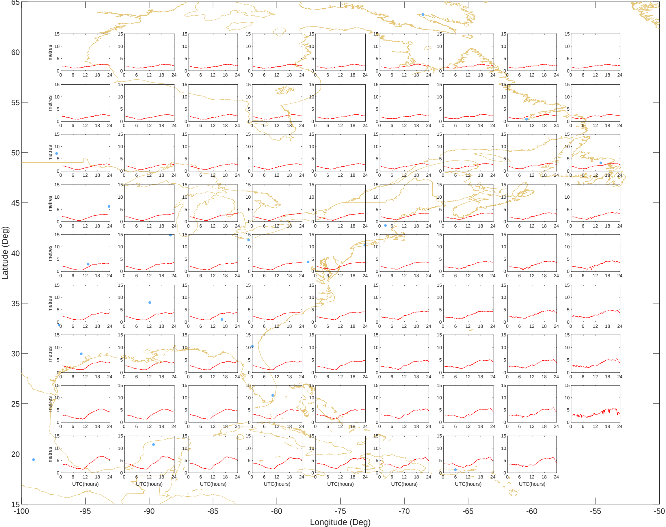
Ionospheric Grid Delays - East (05-Jul-2026) @UNB-WAASLAB
