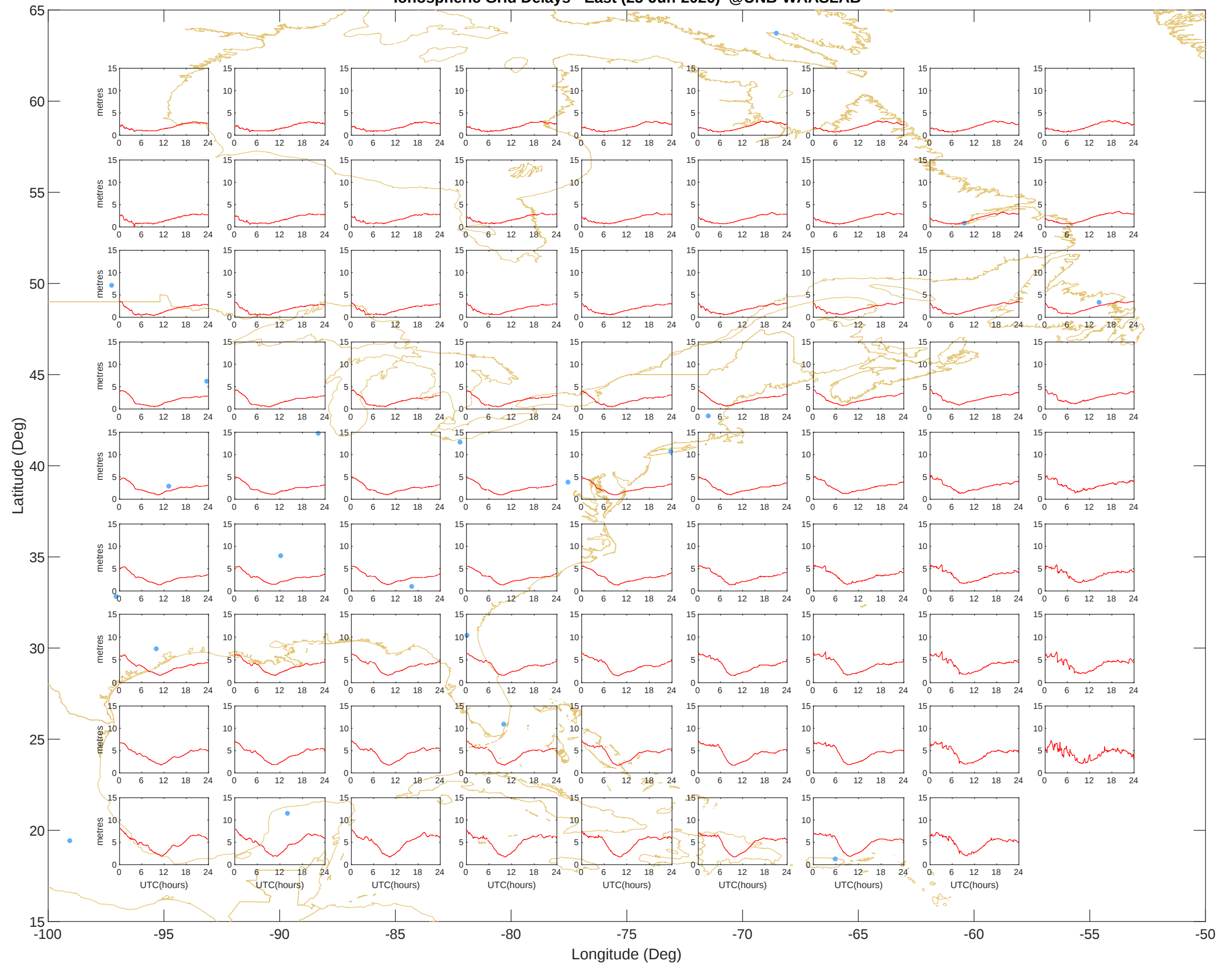
Ionospheric Grid Delays - East (25-Jun-2026) @UNB-WAASLAB
