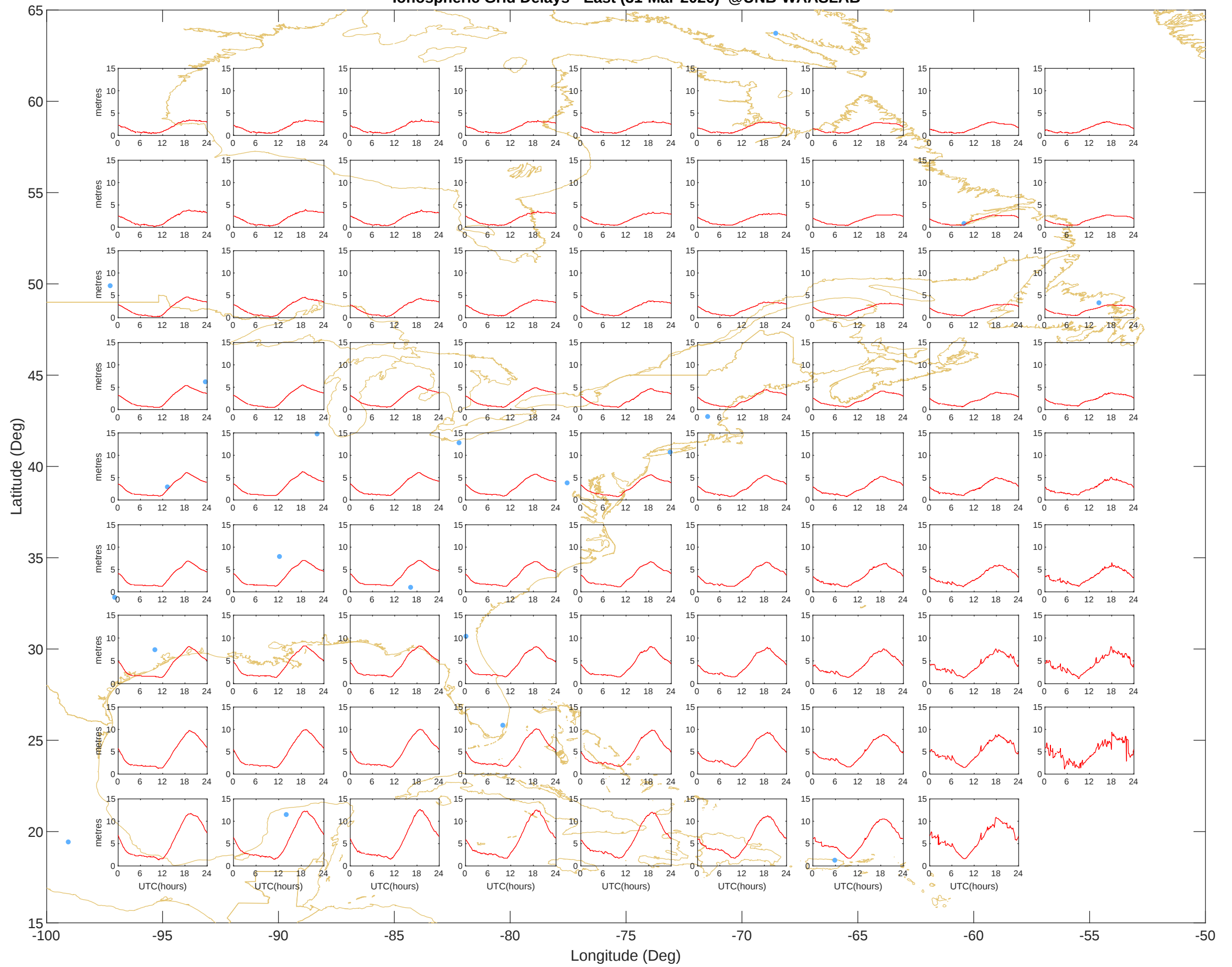
Ionospheric Grid Delays - East (31-Mar-2026) @UNB-WAASLAB
