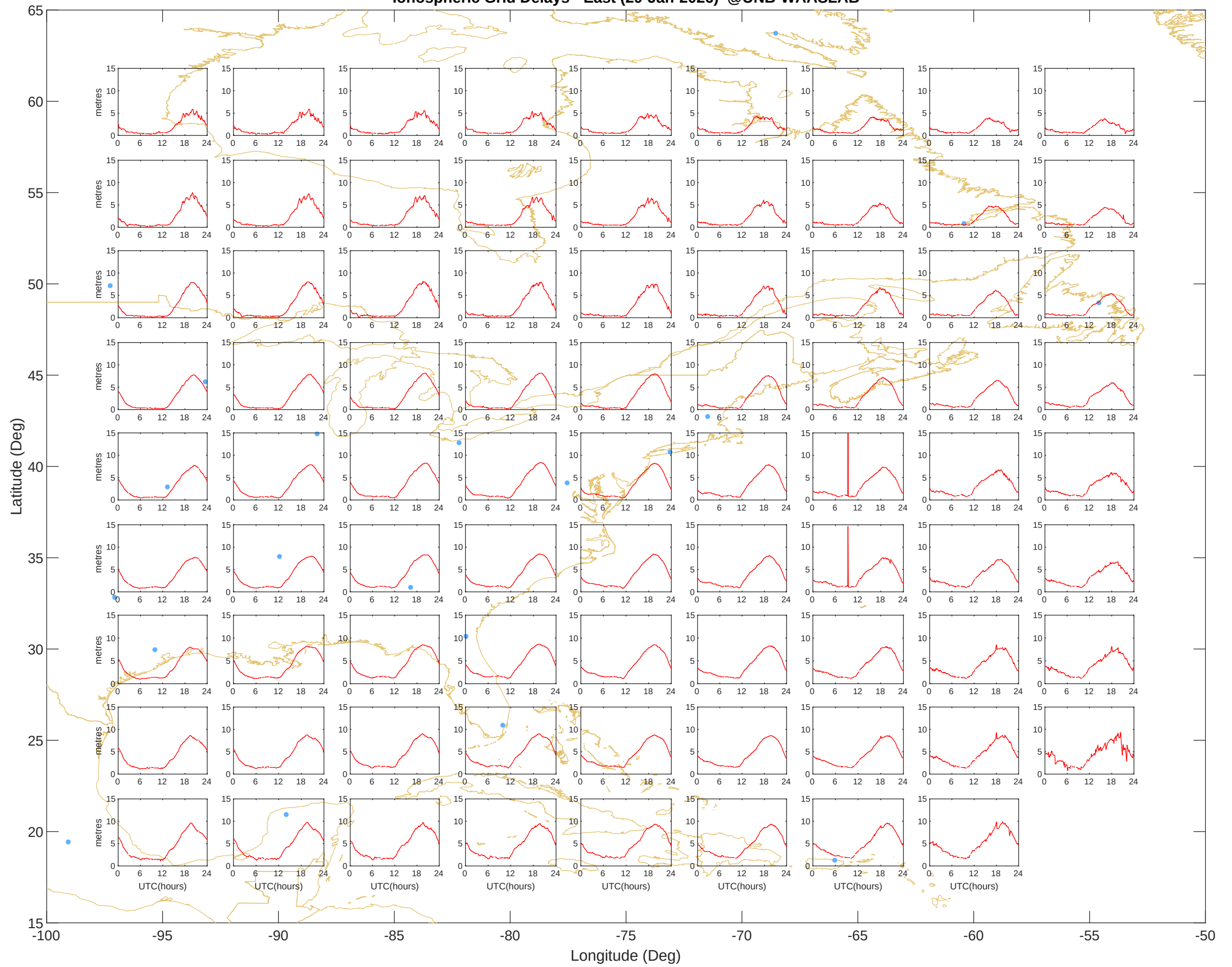
Ionospheric Grid Delays - East (29-Jan-2026) @UNB-WAASLAB
