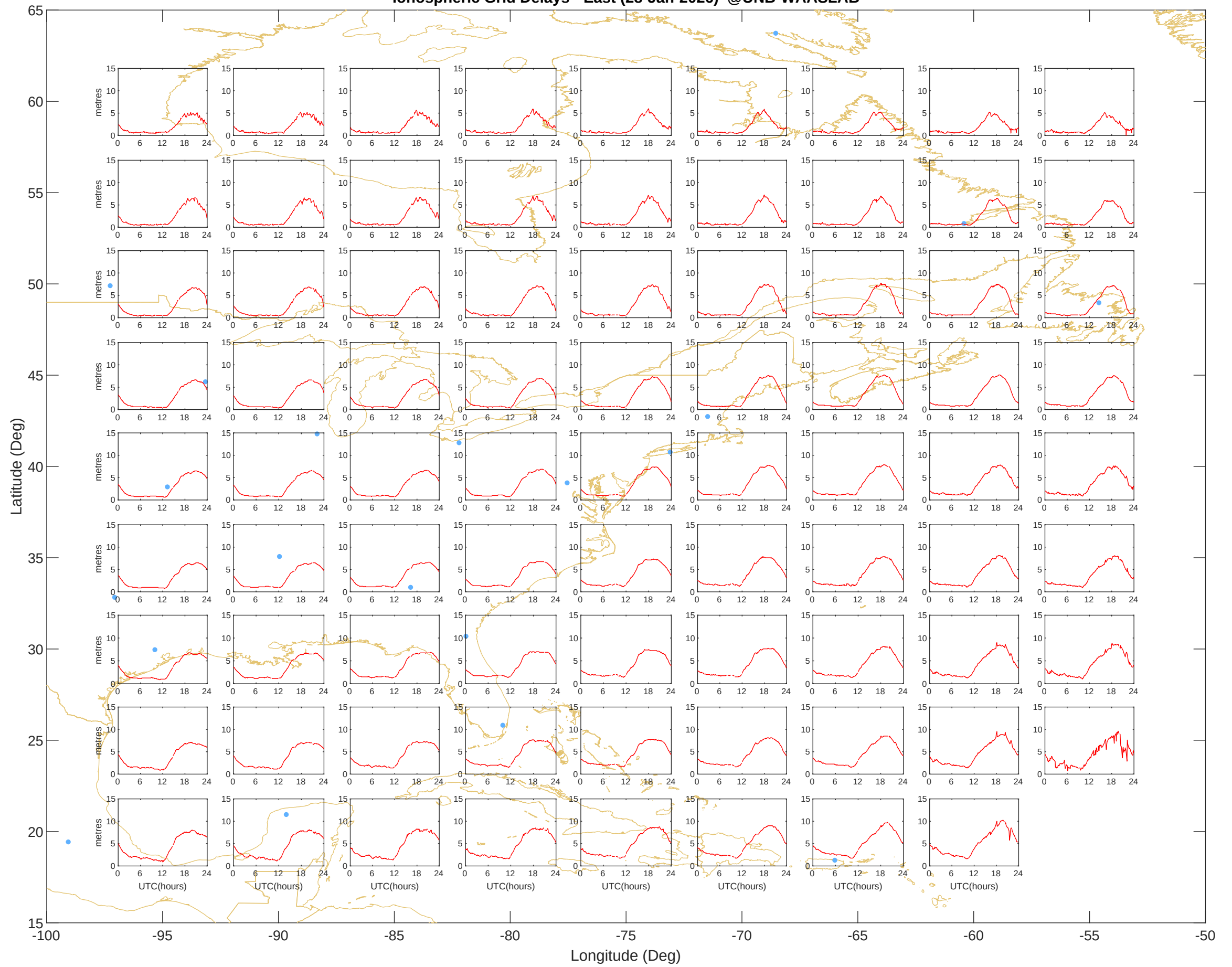
Ionospheric Grid Delays - East (28-Jan-2026) @UNB-WAASLAB
